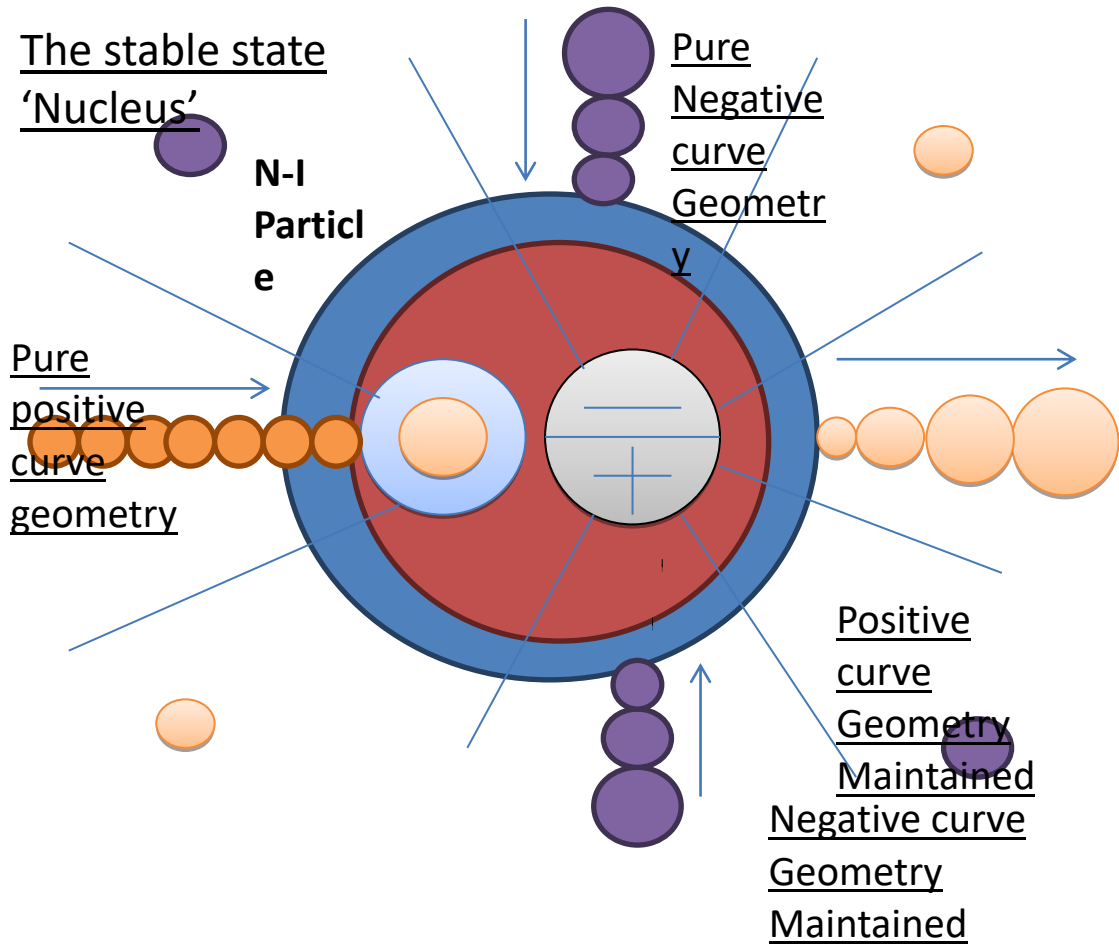
This is the figure of stable state' nucleus and atom.
