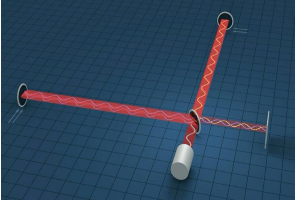
This is the LIGO Experiment BY which Gravitational waves was detected shows same structure as above structure of Nucleus and atom according to Non-Interactive Mechanics.
