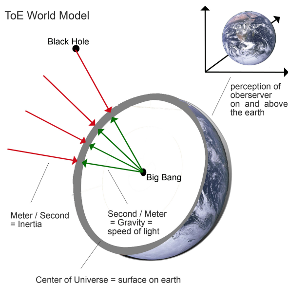
Figure 3 : Surface of earth is center of Universe in regards to “Gravity”. In regards to concept “mass”, there is E_{inertia} = -mc^2 and E_{gravity} = mc^2 . The total Energy on Mass in Universe sums up to Zero.
