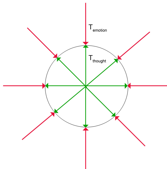
Figure 1 : Gravitational Field = Electromagnetic Field in 2 Dimension representing the Unified F orce that is gravity as inverse proportional inertia from the center of creation (Big Bang)
