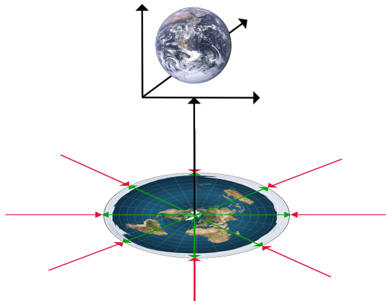
Figure 2 : Flat Earth representing the electromagnetic field as base for projection into 3 dimensional space due to ordering pictures in brain (imaginary time = order).
