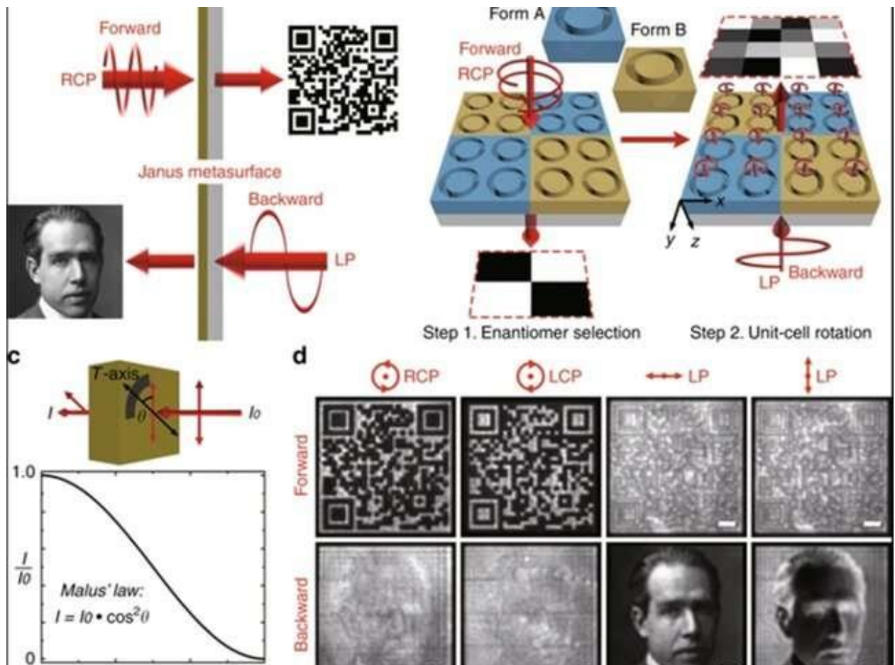
Direction-controlled polarization-encrypted data storage with the Janus metasurface. (a) A schematic diagram of the Janus metasurface for direction-controlled polarization-encrypted data storage. (Photograph used with permission: Niels Henrik David Bohr (1885–1962) Danish physicist. Quantum Theory. Nobel prize for physics 1922/Universal History Archive/UiG/Bridgeman Images.) (b) An illustration of the metasurface encoding process with the two nanoaperture enantiomers having specified rotation angles. (c) The normalized transmission intensity of LP light in the backward direction, which follows Malus's law with respect to the angle \theta between the incident polarization direction and the transmission axis of the 3D helical nanoaperture. (d) Captured transmission images of the Janus metasurface at 800 nm in both the forward and backward directions for various incident polarizations. Scale bar: 10 \mu\text{m} . Credit: Light: Science & Applications, doi: 10.1038/s41377-019-0156-8
