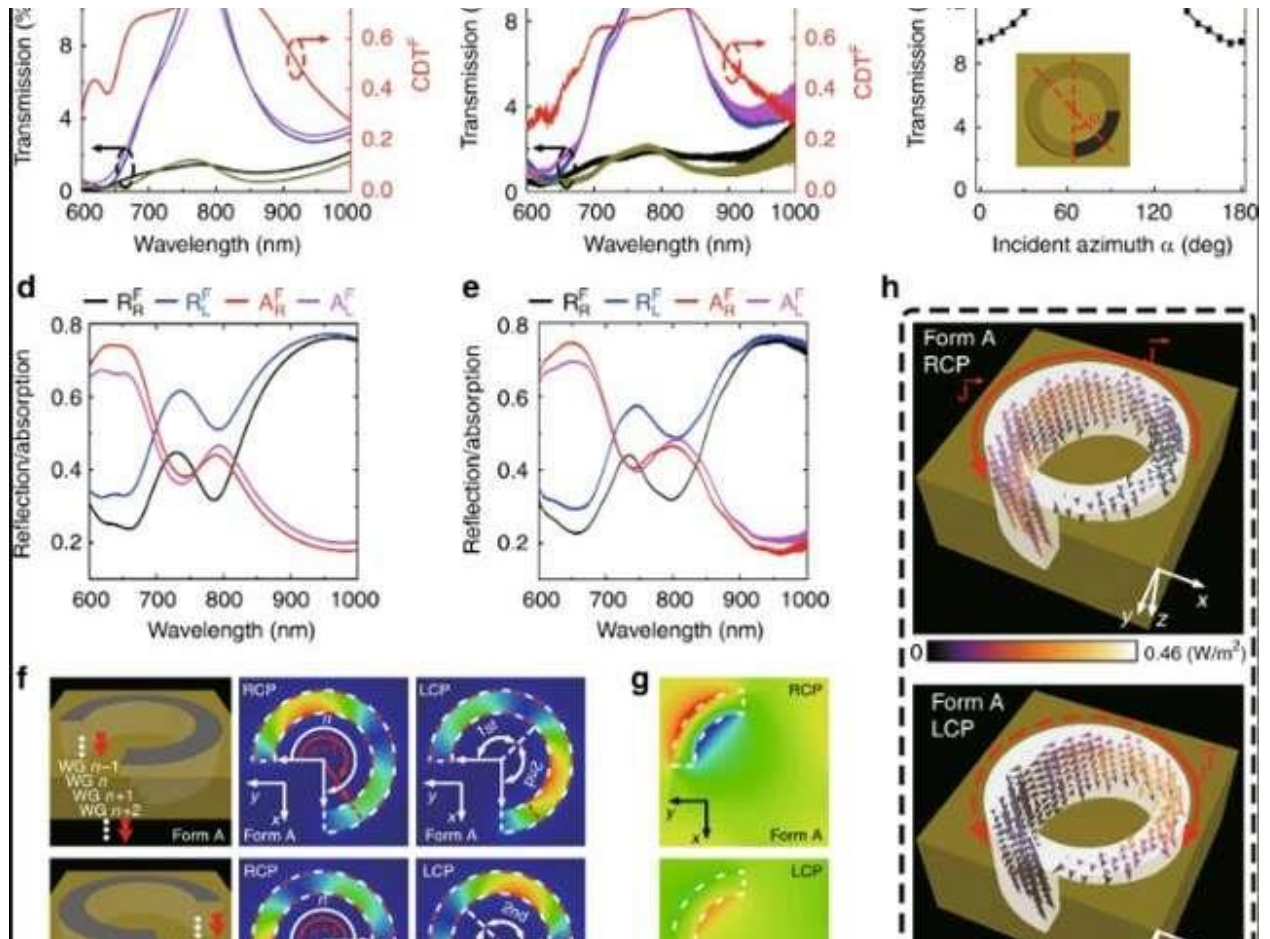
Optical properties of the 3D Janus plasmonic helical nanoaperture in the forward direction. (a) Simulated and (b) measured transmission spectra of the helical nanoaperture array in Form A for various incident/output handedness combinations in the forward direction, together with the corresponding CDTF spectra. (c) The measured transmission intensity as a function of the azimuthal angle \alpha of the LP incident light at 830 nm. (d) Simulated and (e) measured reflection spectra and absorption spectra under RCP (right-handed circularly polarized) and LCP (left-handed circularly polarized) incidence in the forward direction. (f) Illustrations of the spin-dependent mode coupling processes inside the 3D helical nanoapertures in Form A and Form B, which can be considered as series of cascaded waveguide segments (WG n-1 , WG n , WG n+1 ,...). Circularly dichroic mode distributions are presented inside the waveguide segment WG n at 812 nm. (g) Electric field distributions 6 nm above the exit plane of the helical nanoaperture in Form A under RCP and LCP incidence at 812 nm. (h) Optical power flow distributions inside the helical nanoaperture in Form A under RCP and LCP incidence at 812 nm. Credit: Light: Science & Applications, doi: 10.1038/s41377-019-0156-8
