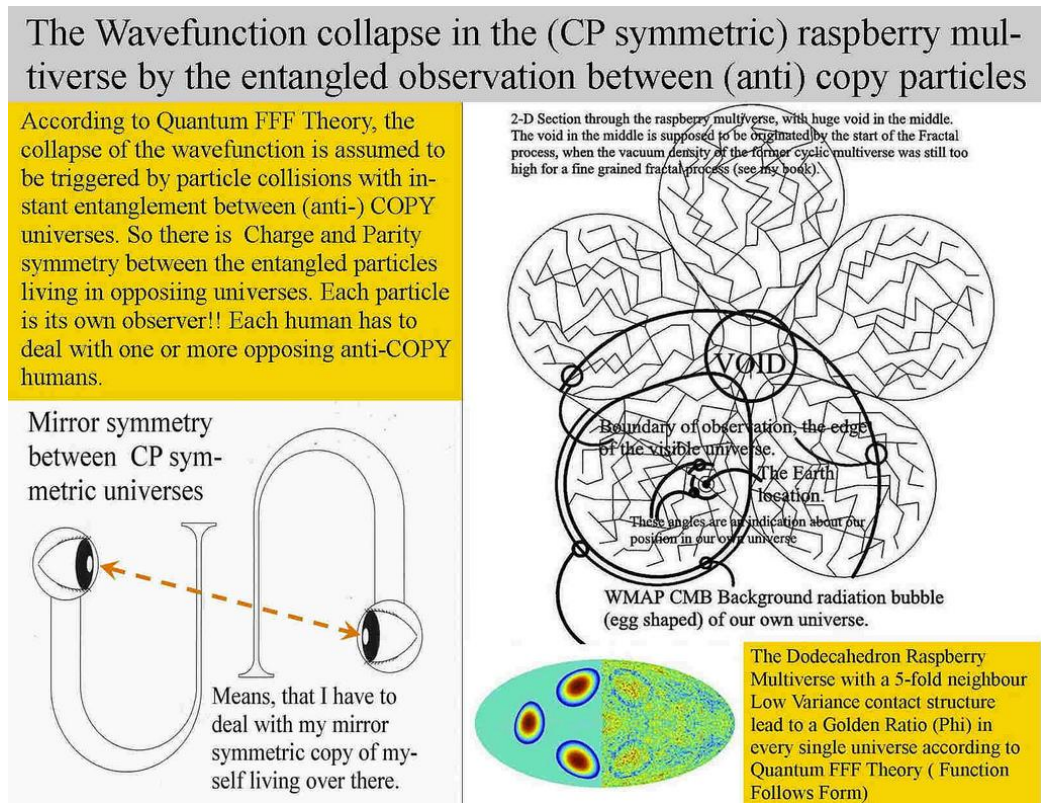
Figure 2, Wavefunction collapse in the Charge Parity ( Time) symmetric Raspberry multiverse.
