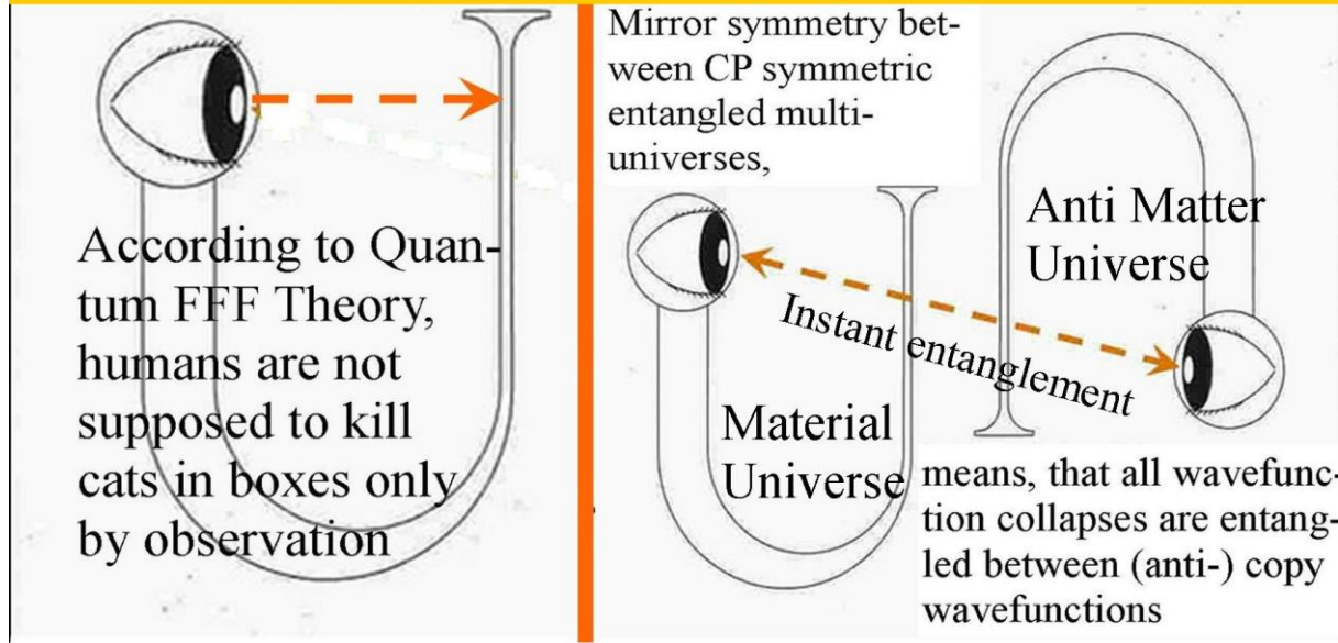
Figure 6, The Alternative QM Theory.
