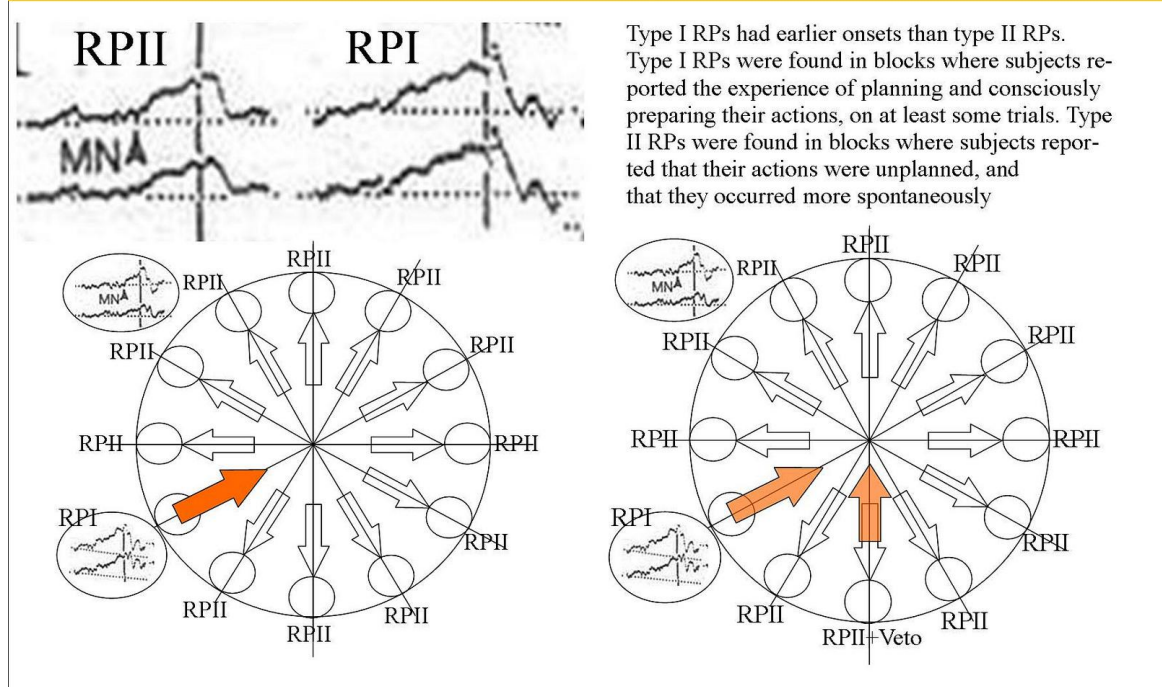
Figure 5, Preplanning (RPI) and (instant Veto/or acceptance) reaction (RPII) represented for a 12 fold multiverse.
