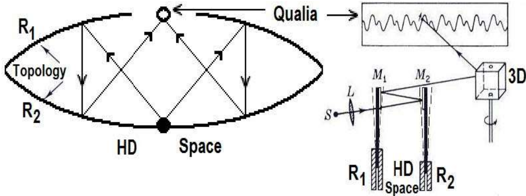
Figure 2. 2D rendition of a nonlocal 12D holographic process. A quale object (black circle) placed inside (LCU array) two parabolic mirrors produces a virtual image (white circle) representing creation of a point in spacetime. Our 3D virtual holographic reality is produced in a similar fashion by future-past standing-wave (R1-R2) parameters from the Higher Dimensional (HD) mirror symmetric infinite potentia of the Unified Field, UF . This same process produces (evanesces) qualia with each lit point (white circle) like raindrops producing a rainbow from sunlight (noeon field).
