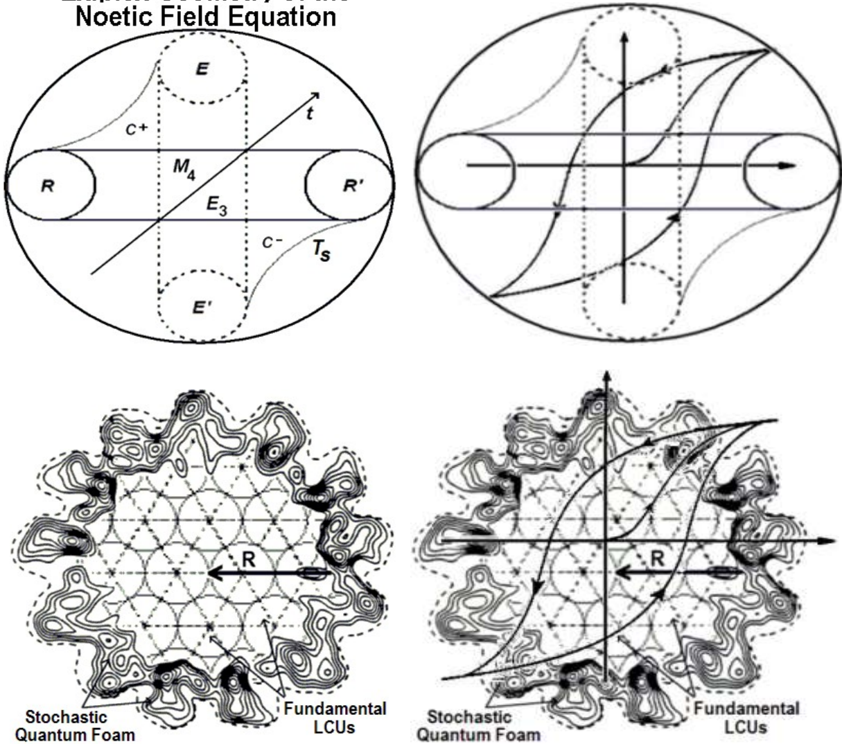
Figure 5. a) A hysteresis loop is added to Figs. 1c & 3a. Geometric metaphor for Noetic Field Equation. b) Overlap of a hysteresis loop with action of the noetic field. c) Psychon-dendron coupling. d) Overlap of hysteresis loop with psychon-dendron interaction.
