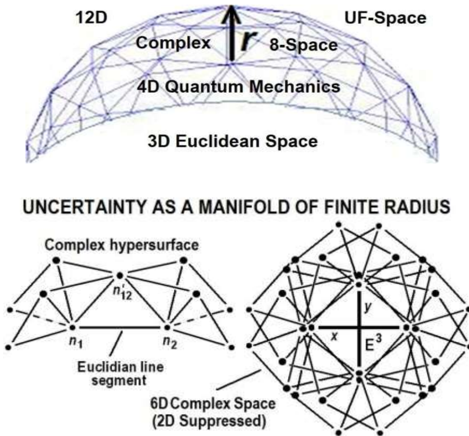
Figure 9. Proposed 2D to 5D Manifold of Uncertainty (MOU). a) Partial hyperspherical view. b) Suppressed planar views.
