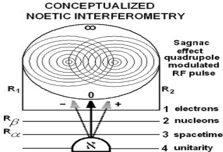
Figure 11. Conceptualized Riemann sphere Cavity-QED multi-level Sagnac effect interferometer designed to ‘penetrate’ spacetime emitting the ‘eternity wave, \aleph ’ of the UF .
