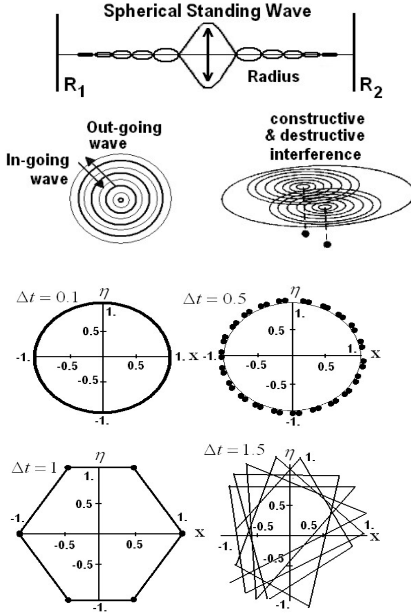
Figure 8. The Dirac polarized vacuum has hyperspherical symmetry. a) Top left, metaphor for Cramer’s standing-wave present showing future-past elements, R_1, R_2 , 11D of 12D suppressed for simplicity. b) Bottom left, top view of a) 2D spherical standing-wave; c) Bottom left right portion, manipulating relative quantum/brane phase oscillations creates nodes of destructive and constructive interference. d) Right, Four numerical simulations of the phase space trajectory of the Dubois superposed incurvise oscillator based on coordinates and velocities x_n = 1/2[x_n(1) + x_n(2)] v_n = 1/2[v_n(1) + v_n(2)] shown in the figure for values of \Delta \tau = \omega t equal to 0.1, 0.5, 1.0 and 1.5. Initial conditions are \chi_0 = 1, \eta_0 = 0 & \tau_0 = 0 with total simulation time, \tau = \omega t = 8\pi .
