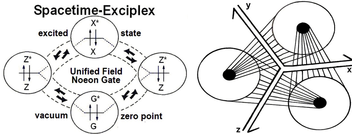
Figure 4. a) Proposed HD Exciplex Properties of Spacetime synonymous with the gating action of the UF equation (Fig. 3a) and the hysteresis Psychon filling of a dendron (Fig. 3b). The four circles represent spacetime LCUs (Fig. 4b). In the Standard Model with a ZPF ‘basement of reality’ (G in the Figure) Psychon energy could not form a hysteresis loop because excitation of the ZPF to Z elements in the Figure could only occur for the brief Planck time. But since the exciplex never goes to ground, (see text) an exciplex LCU structure acts as a gate allowing UF energy to be ‘pumped’ into a dendron. b) Complex 3-fold LCU fermionic vertex, x,y,z. Each X,G,Z circle (not shown in 4a) is one triune LCU as in b. The circles in Figs. 3a and especially Fig. 1c each represent one LCU.
