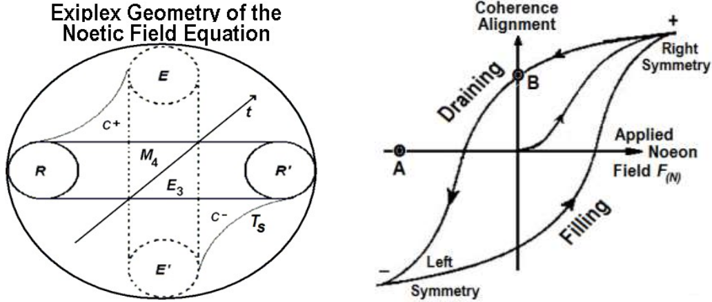
Figure 3. a) Geometric topology of Noetic Field Equation F_{(N)} = E/R acting as a holophote (rotating lighthouse beacon) gating mechanism for entry of the nonlocal HD UF into local M_4-E_3 3(4)-space. Wave-particle-duality is elevated to a principle of cosmology such that the solid bar, R_1-R_2 at one moment transforms to the dotted bar, E-E' at the next in a continuous relativistic wave-particle cycle with t the arrow of time. \pm C^4 is a complex 8-space and T_S fluctuating string tension helping drive the oscillation. b) UF Hysteresis Loop. Point A is a Zero-point where the driving field reverses and increases. Point B is where the driving field drops but still retains considerable charge as a UF force of coherence related to the life-principle and quale.
