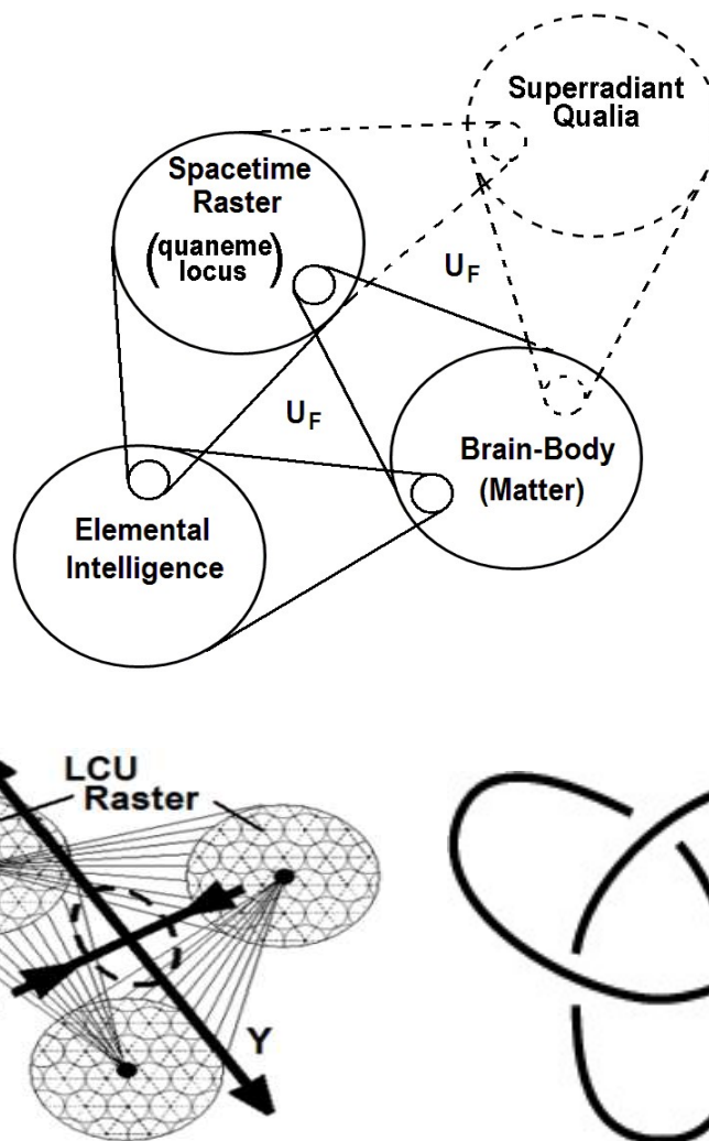
Figure 7. a) Physical basis of continuous superradiant generation of qualia from three components of mind: eternal Elemental Intelligence, Brain-Body (Descartes res extensa ), and the Superradiant Qualia (Descartes res cogitans ) mediated by the spacetime raster (quaneme locus) that exciplex gates ‘light of the mind’ or U_F energy. The term quaneme is derived to parallel phoneme component of sounds. b) LCU construct of hidden nonlocally behind a 3-space singularity (black cross vertex). c) Trefoil able to transform into a circle.
