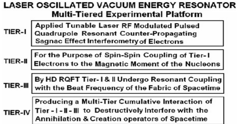
Figure 10. Design elements of the Noetic Interferometer postulated to constructively-destructively interfere with the topology of the spacetime manifold to manipulate the UF . The first three tiers set the stage for the critical 4 th tier which through an incursive oscillator punches a hole in the fabric of spacetime creating a holophote entry of the UF into the experimental apparatus.
