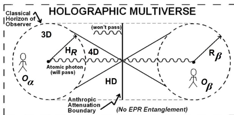
Figure 3. Illustrating how the quantum uncertainty principle blocks the experience of spiritual entrainment between souls (or God) relative to 3-space. The attenuation boundary (center) expands from conic closed (shown) to parallel (open) when sensory awareness uncouples from 3-space and recouples to 12D spiritual-space during entrainment in a mystical experience.
