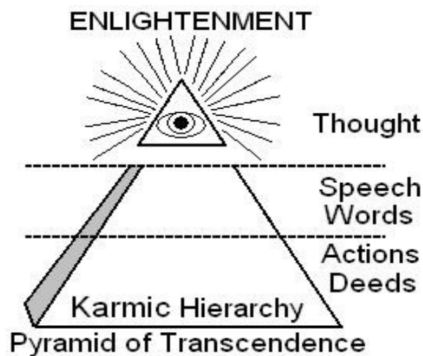
Figure 4. Pyramid of Transcendence / enlightenment. Individuals Living operationally at the top of this karmic pyramid spontaneously develop transcendent abilities. Sin or violation of ethical principles, commandments or Karmic law can be classified into three weighted categories of decreasing severity: 1. Actions, 2. Speech, 3. Thoughts.
