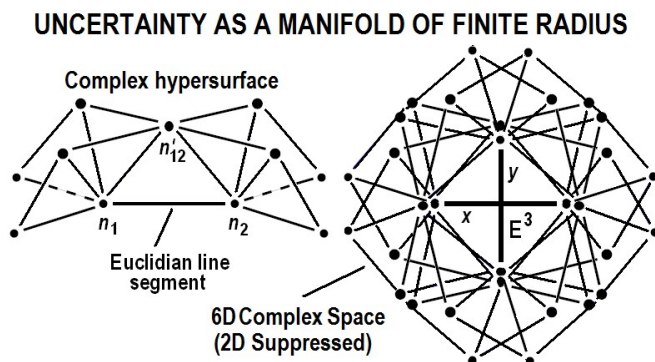
Figure 1. Conceptual view of the manifold of uncertainty with 64 cyclic quaternionic elements (some suppressed) with Euclidean 3-space, E_3 as the resultant subspace of virtual 0D points forming observed reality. a) 1D line element between two points illustrating HD elements hidden behind the quantum uncertainty principle. b) Additional 6D mirror symmetric elements forming the finite radius manifold of uncertainty, beyond which a physically real parameter of the unified field, a life-principle synonymous with the spirit of God exists in an infinite multiverse.
