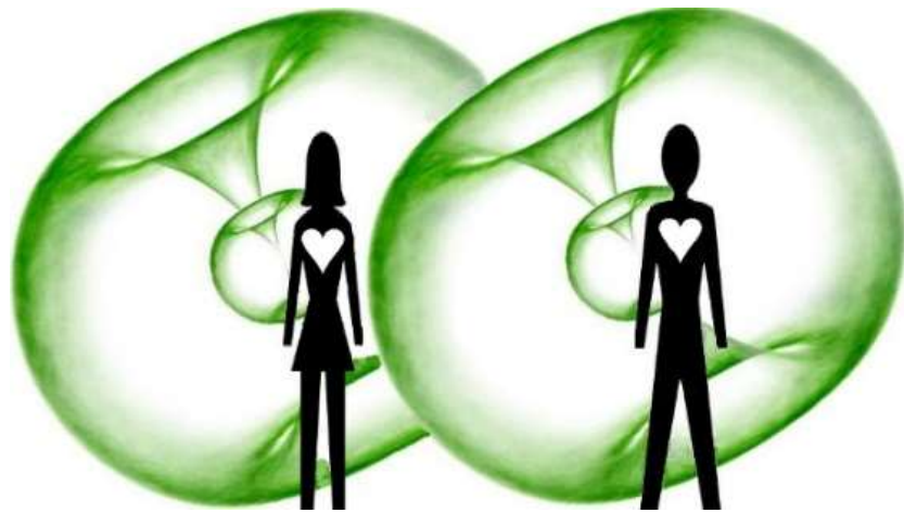
Figure 7. When SOLS align, a coupling of the noetic field occurs resonating between the two souls allowing them to share the mutual entangled qualia of love. While the hypertori images are illustrative here; the actual psychosphere structure and hyperspherical topology has some similarities, i.e. wheels within wheels with gating mechanisms that may align or misalign.
