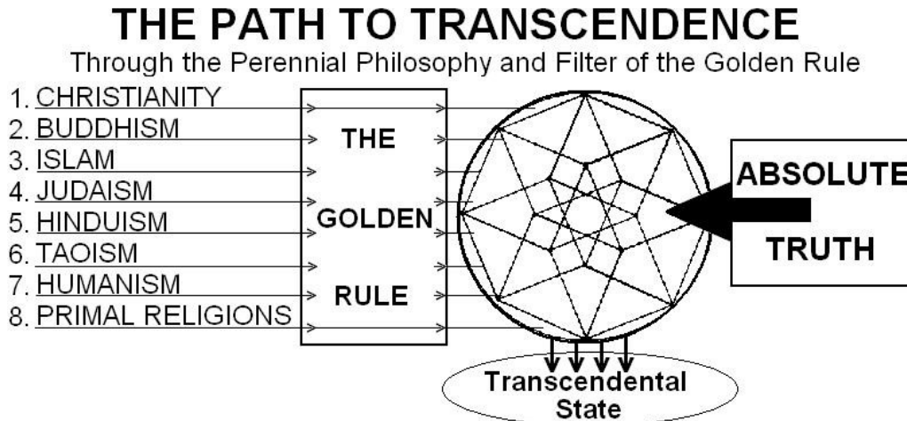
Figure 5. Because of the inherent spiritual nature of mankind in an Anthropic Cosmology with a Cartesian teleological life principle and the concomitant existence of Absolute Truth in regard to spiritual matters, the Golden Rule, as a universal principle of the Perennial Philosophy, provides a path to both find God and spontaneously develop transcendence in the process.
