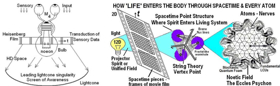
Figure 2. Metaphors of sensory transduction and entry of life principle into living systems across the Cartesian mind-brain barrier becoming qualia a), and infused into biochemistry in b).
