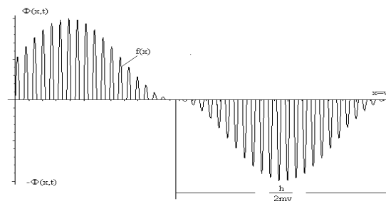
Fig. 2. Behavior of wave packet in linear dispersion medium (i.e., rather like a series of stroboscopic photographs).
