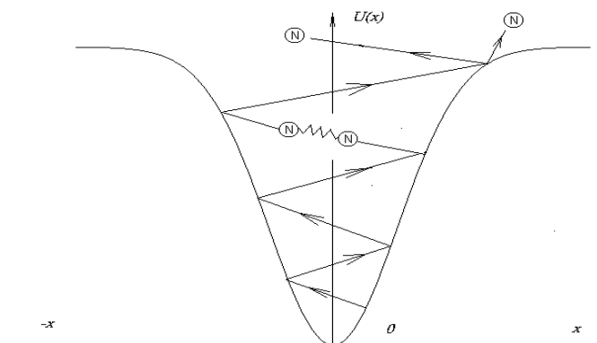
Fig.8. Oscillation of Nitrogen molecule in potential well of catalyst.
