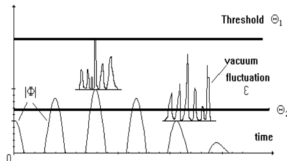
Fig.4. Quantum measurements.
