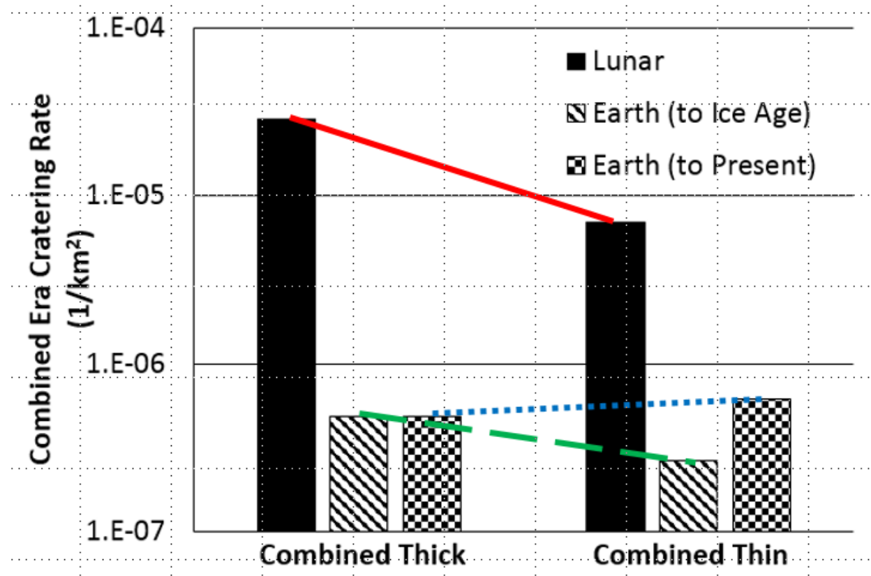
Figure 4. Comparing Trends in Cratering Rates for the Earth and Moon over the Combined Thick and Thin Atmosphere Eras
