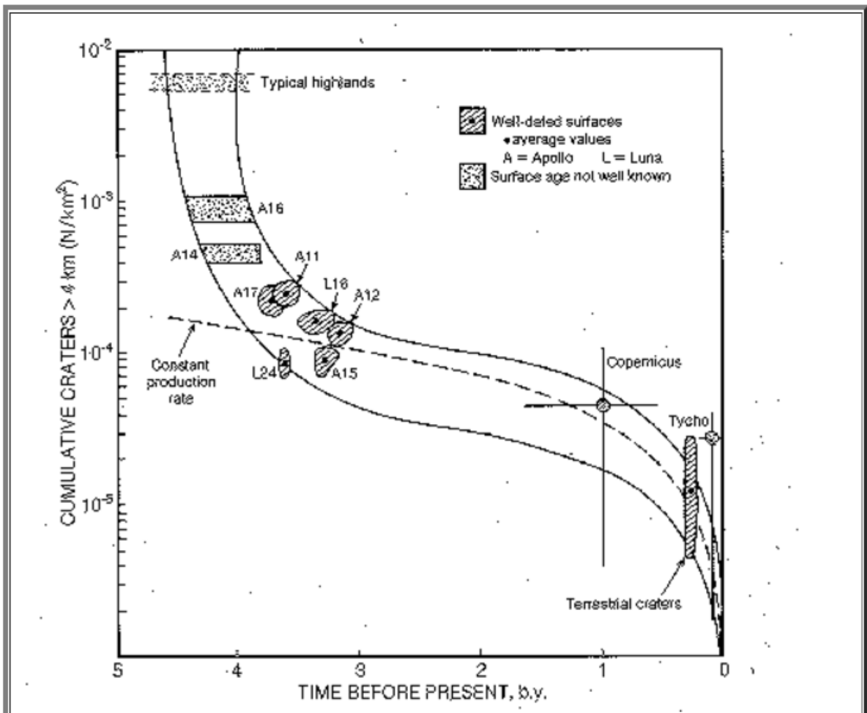
Figure 1. Lunar crater production rates through geologic time as reconstructed from the measurement of crater densities on the lunar surface and from absolute age dating of returned lunar rocks. Firm correlations can only be reconstructed for (1) the well-characterized basalt surfaces (3.8-3.2 Gyr) and (2) the contemporary meteorite flux based on current astronomical observations ( t = 0 ). The ages of Tycho and Copernicus are inferred from indirect evidence. From F. Horz et al. p.84.
