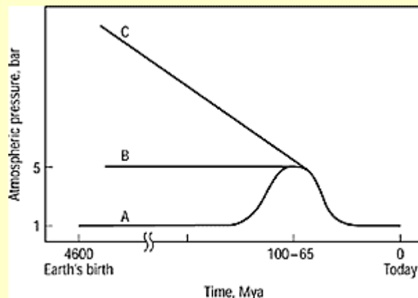
Figure 1. Three possible alternatives for the atmospheric pressure early in Earth’s lifetime, given that it was at ~5 bar, ~100 Mya.
