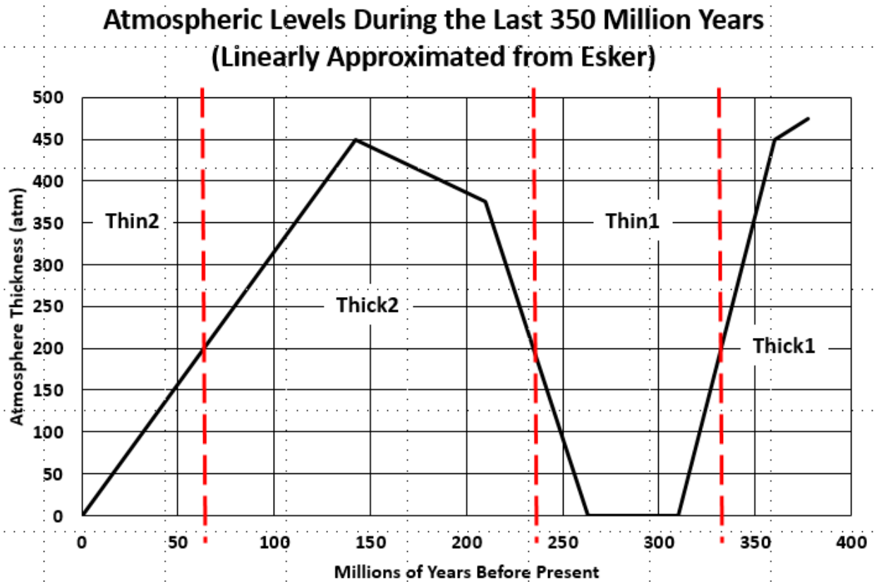
Figure 2. Atmospheric Levels during the Last 350 Million Years with Assumed Transition Times
