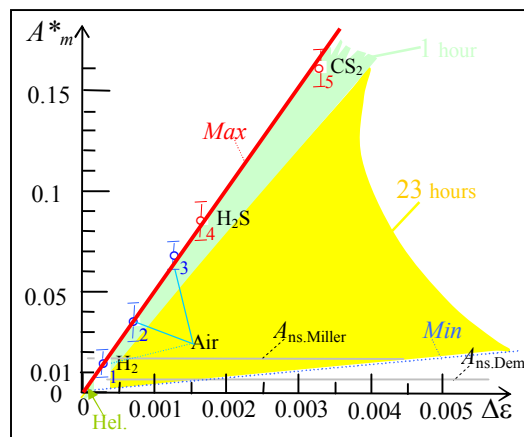
Fig.1. The dependence of the A_m(\Delta\varepsilon) amplitude A_m of the interference fringe shift from the polarization contribution \Delta\varepsilon_{\text{pticl.}} particles to the total permittivity \varepsilon=1+\Delta\varepsilon_{\text{pticl.}} light-carrying medium the Michelson interferometer (MI), discovered by me in 1968 (for l_{\parallel}=l_{\perp}=7 m, and \lambda=6\cdot 10^{-7} m) [3]:
