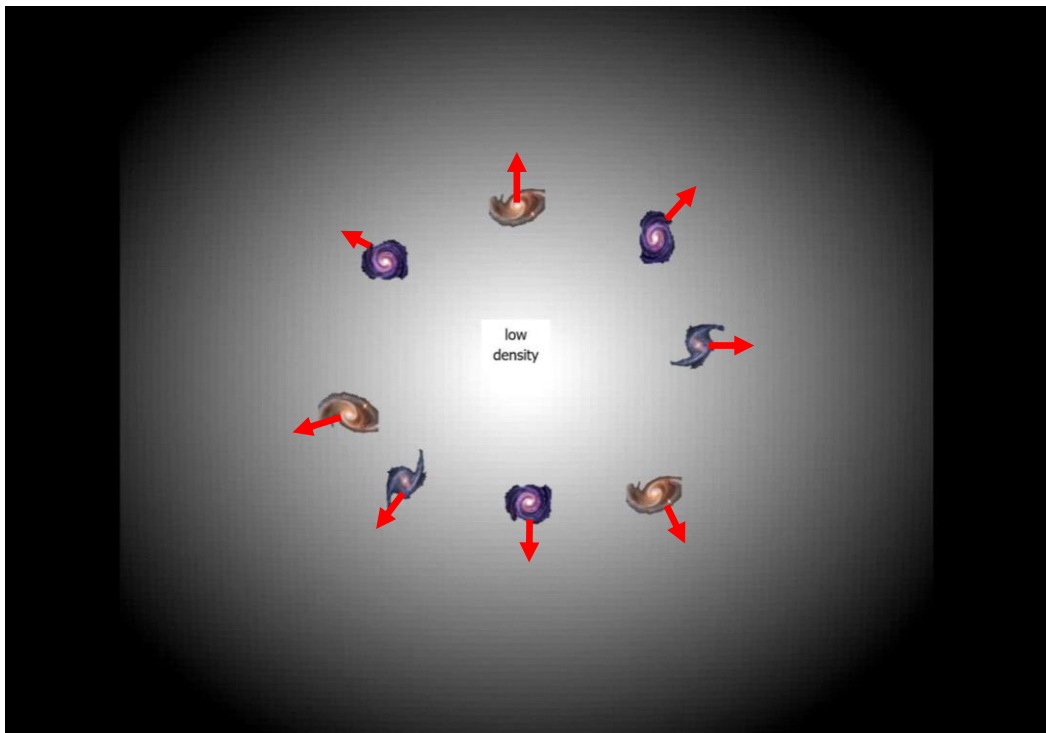
Fig. 3. A zone with a lower density of primary substance results in an inverse gravitational field, and stars and galaxies are accelerated outward.
