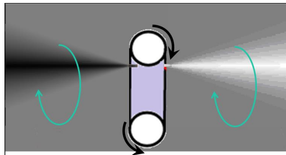
Fig. 4. Illustration of the charge of an electron. The gray shading shows the change in the medium density caused by the behavior of the electron vortex. The electron is shown schematically as a cross-section.
