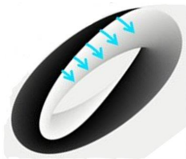
Fig. 8. Any fragment of a vortex particle is a density wave. The arrows show the direction of the density wave velocity as part of the electron vortex.
