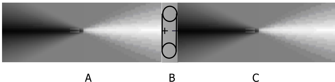
Fig. 6. The medium density created by the charges of electrons A and C (electrons A and C themselves are not shown). The force on electron B has the same origin as the gravitational force.
