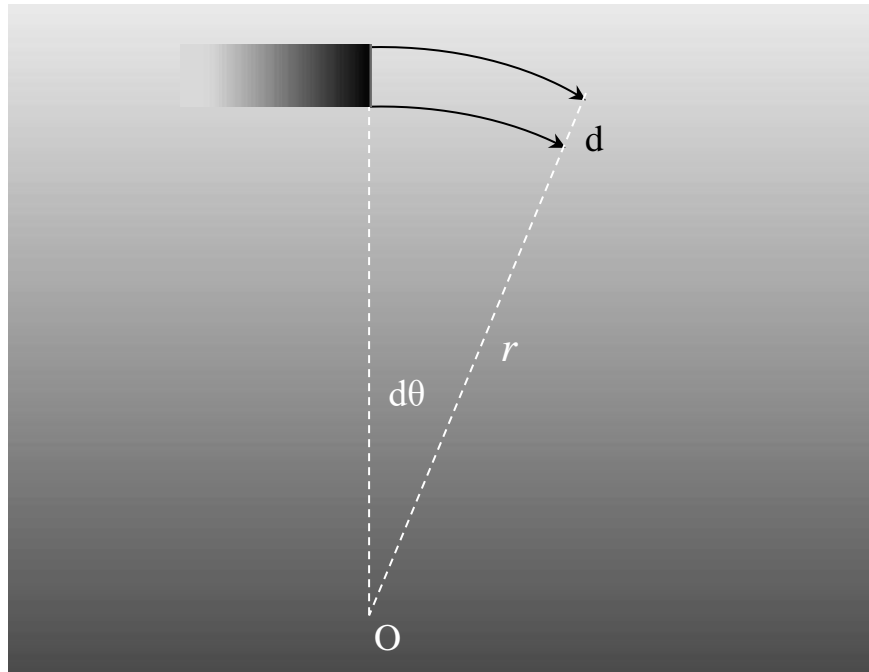
Fig. 7. A density wave of the primary substance is deflected in a gravitational field toward the region of higher density.
