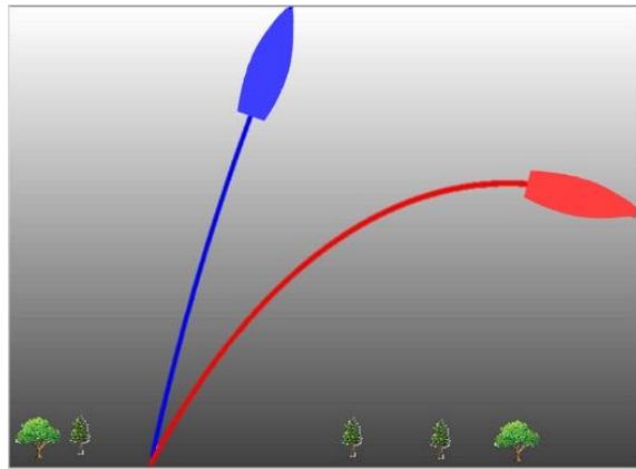
Fig. 10. Two possible trajectories of a rocket.
