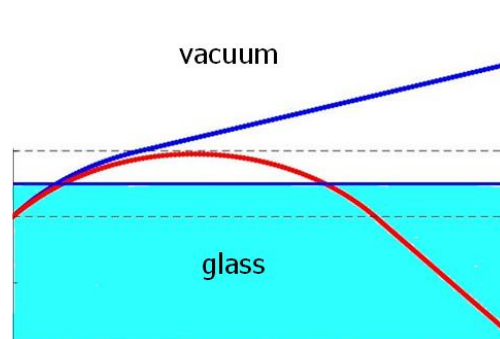
Fig. 9. Two possible trajectories of a photon: refracted (blue) and "reflected" (red). The glass/vacuum boundary layer is shown by a dotted line.
