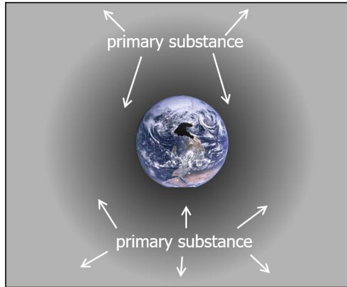
Fig. 1. This figure shows the planet Earth, surrounded by the primary substance. Although the primary substance is not visible, it is depicted in shades of gray in this figure; the darker color corresponds to a higher density of the primary substance.
