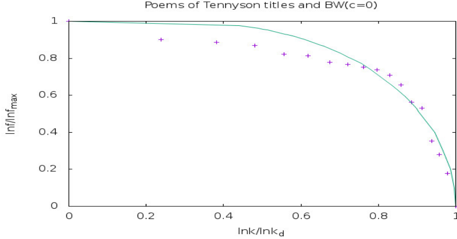
FIG. 3. Vertical axis is \frac{\ln f}{\ln f_{max}} and horizontal axis is \frac{\ln k}{\ln k_{lim}} . The + points represent The Poems of Tennyson titles, with the fit curve, BW( c=0 ), being the Bragg-Williams curve in the absence of external magnetic field, c = \frac{H}{\gamma\epsilon} = 0 .
