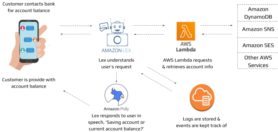
Figure 5: Workflow of getting banking information through a Chatbot
