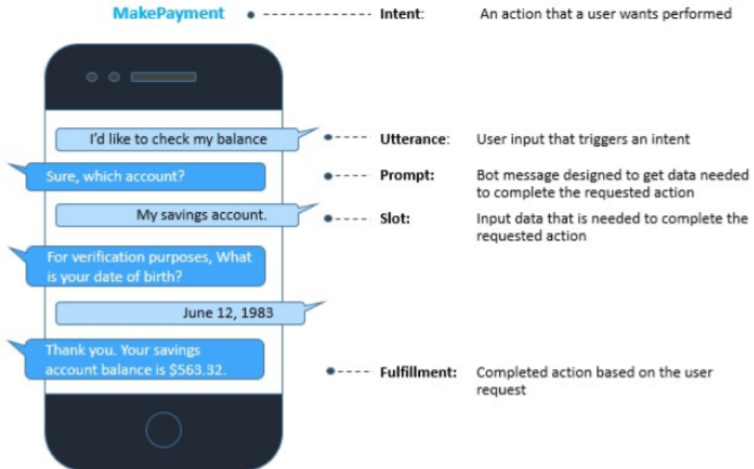
Figure 6: Preview of Flow of Conversation
