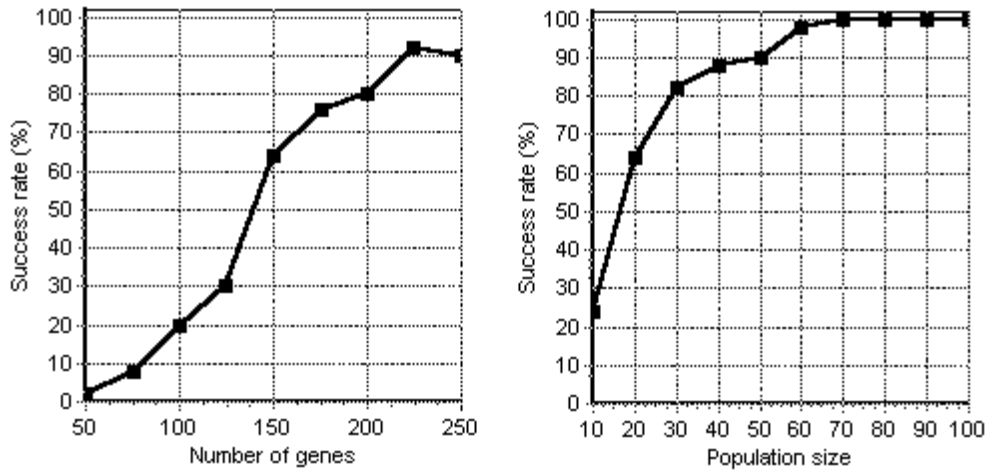
Figure I.10. The relationship between the success rate and the chromosome length (left side) and the population size (right side). Results are averaged over 50 runs.
