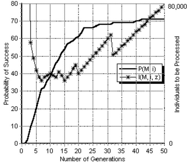
Figure I.7. The computational effort and the cumulative probability of success for the even-5-parity problem. Results are averaged over 100 runs.
