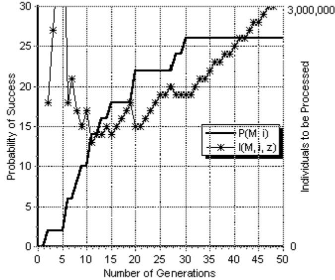
Figure I.5. The computational effort and the cumulative probability of success for the even-5-parity problem.
