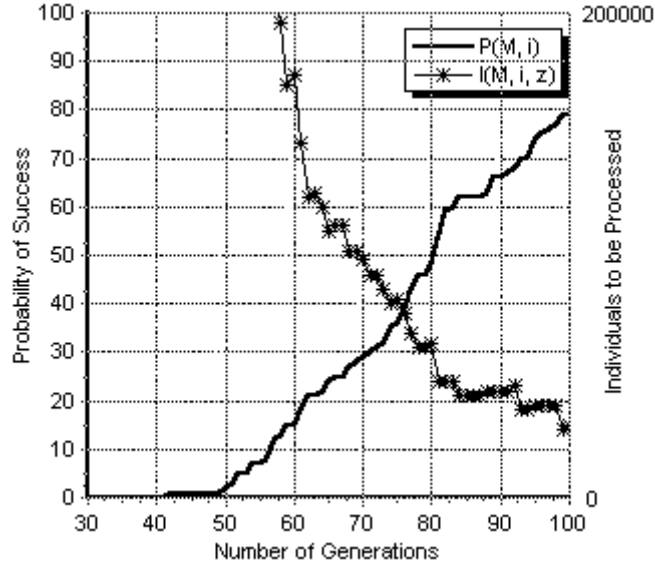
Figure I.14. The computational effort and the cumulative probability of success for the even-15-parity problem. Results are averaged over 100 runs.
