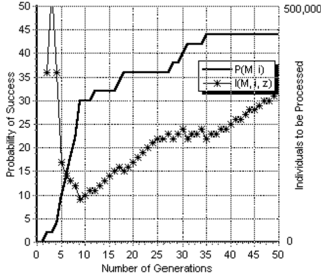
Figure I.8. The computational effort and the cumulative probability of success for the even-6-parity problem. Results are averaged over 50 runs.
