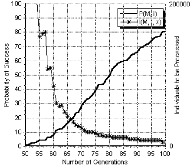
Figure I.11. The computational effort and the cumulative probability of success for the even-12-parity problem. Results are averaged over 100 runs.
