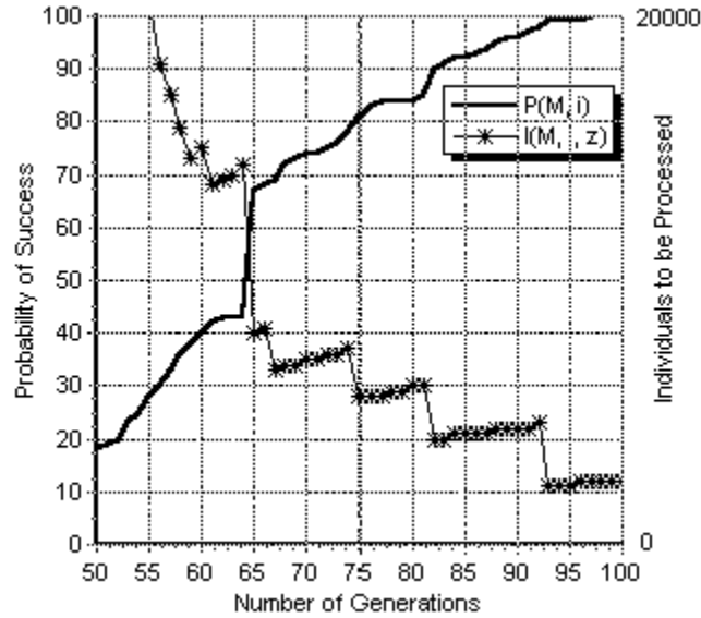
Figure I.12. The computational effort and the cumulative probability of success for the even-13-parity problem. Results are averaged over 100 runs.
