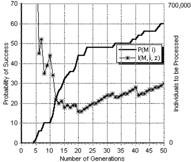
Figure I.9. The computational effort and the cumulative probability of success for the even-7-parity problem. Results are averaged over 50 runs.
