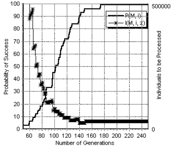
Figure I.15. The computational effort and the cumulative probability of success for the even-16-parity problem. Results are averaged over 100 runs.
