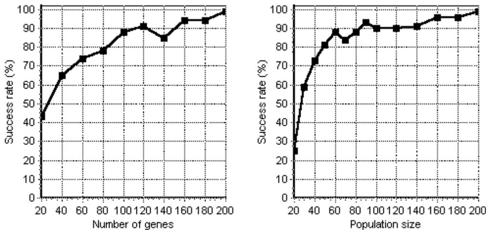
Figure I.6. The relationship between the success rate and the chromosome length (left side) and the population size (right side). Results are averaged over 100 runs.
