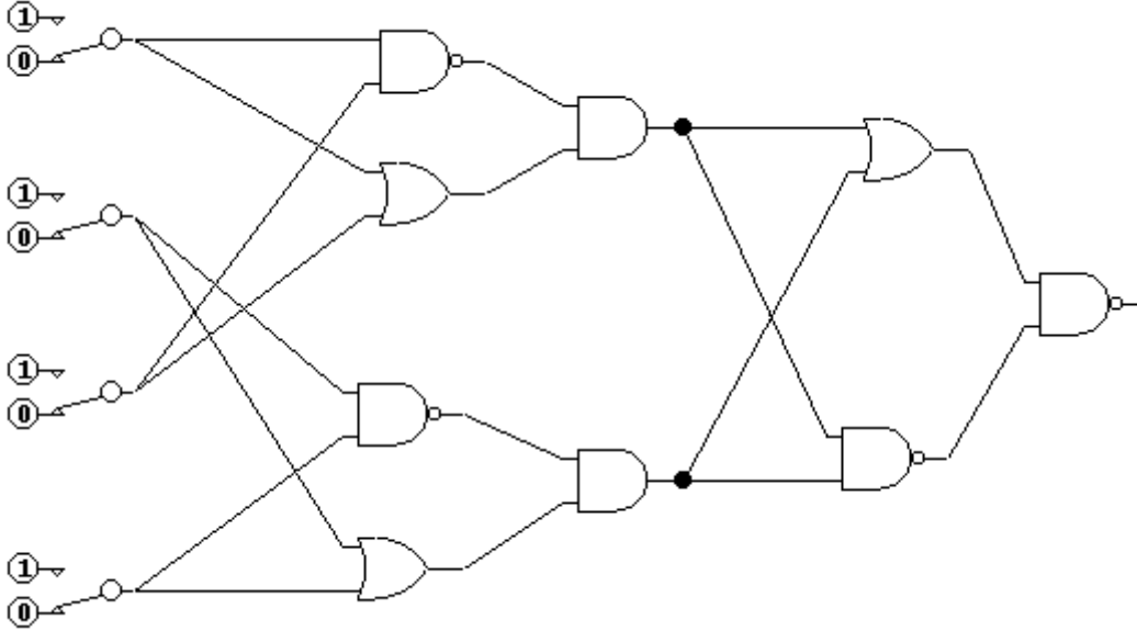
Figure I.4. A circuit for the even-4-parity problem.
