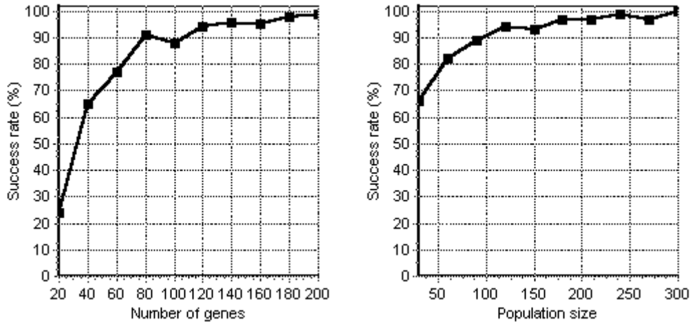
Figure I.1. The relationship between the success rate and the chromosome length (left side) and the population size (right side). Results are averaged over 100 runs.
