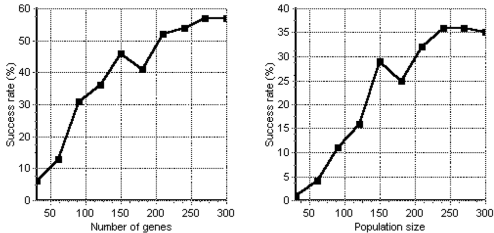
Figure I.3. The relationship between the success rate and the chromosome length (left side) and the population size (right side). Results are averaged over 100 runs.
