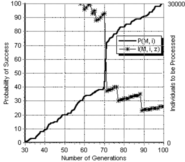
Figure I.13. The computational effort and the cumulative probability of success for the even-14-parity problem. Results are averaged over 100 runs.
