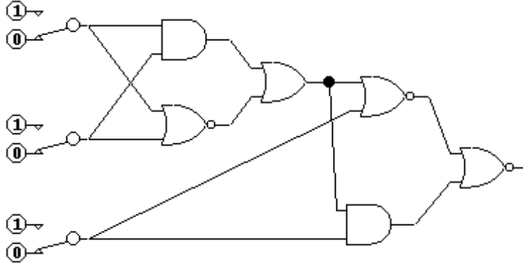
Figure I.2. A circuit for the even-3-parity problem.
