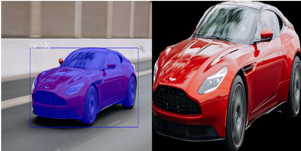
Object Extraction using a pre-trained Mask R-CNN COCO model.
