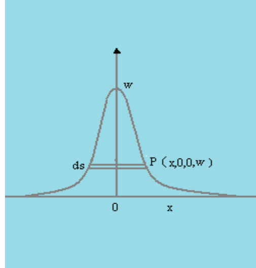
Fig.3: Showing cross section of 4D Gaussian structure by x - w plane
