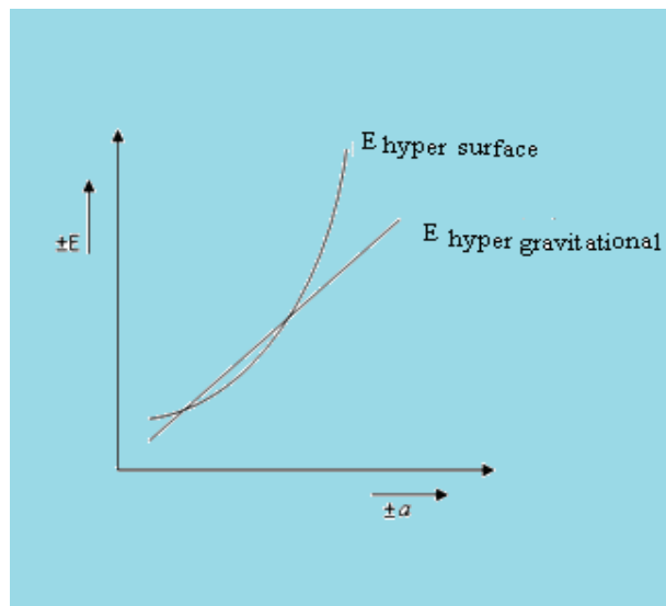
Fig.6 shows equilibrium points where hyper surface and hyper gravitational energy of fundamental particles are equal.
