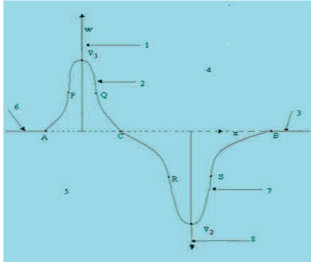
Fig.7 shows cross section of two 4D Gaussian structure of electron-proton pair by x - w plane in a particular state during spiral transformation.
