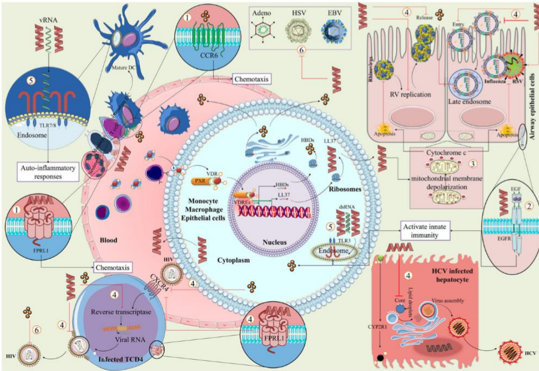
FIGURE 2 Vitamin D and induction of antimicrobial peptides against viral infection. Vitamin D-induced antimicrobial peptides (LL37 and HBDs) via VDR and RXR dimerization act against viral infections through (1) binding to FPRL1 and CCR6 for recruiting immune cells to site of infection; (2) activation of innate immunity by transactivation of the EGFR; (3) clearance of viral infection through mitochondrial membrane depolarization and release of cytochrome c; (4) down-regulation of cell entry, replication, and viral release; (5) protection of viral RNAs from degradation and induced immunity response through TLRs activation; (6) and direct effects on virions. Abbreviation: Epidermal growth factor receptor (EGFR), formyl peptide receptor-like 1 (FPRL1), human \beta -defensins (HBDs), retinoic X receptor (RXR), toll-like receptor (TLR), and vitamin D receptor (VDR)
