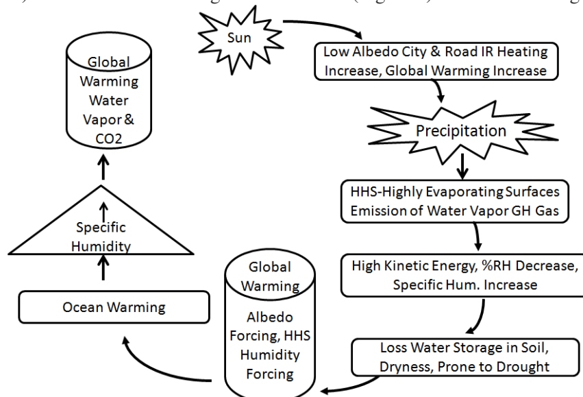
Figure 1A HHF-HHS-HES feedback view of contribution to global warming
