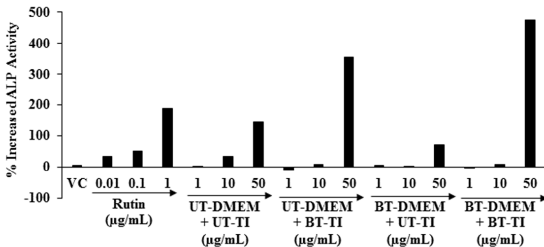
Figure 2. The effect of test samples on alkaline phosphatase (ALP) enzyme activity in human bone osteosarcoma cell (MG-63). VC: Vehicle control (0.05% DMSO), UT: Untreated; BT: Biofield Energy Treated; TI: Test item.
