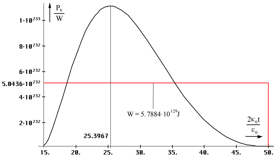
Figure 64 Power dissipation of the Metric line-element during the second maximum
