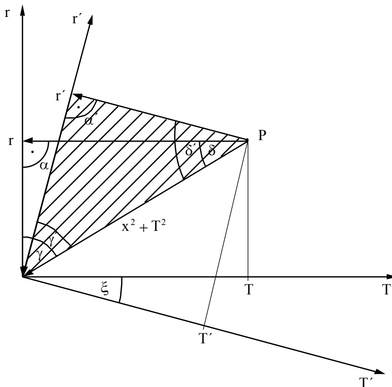
Figure 144 Rotation in the (T, r) -plane during the LORENTZ-transformation
