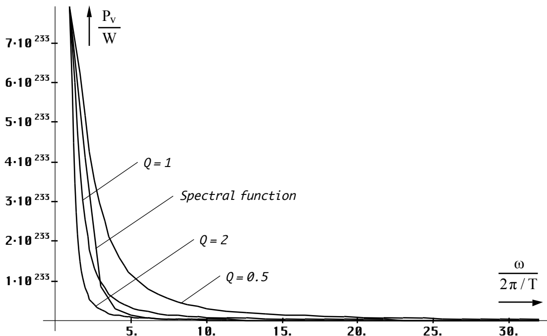
Figure 66 Continuous spectrum (second maximum)
