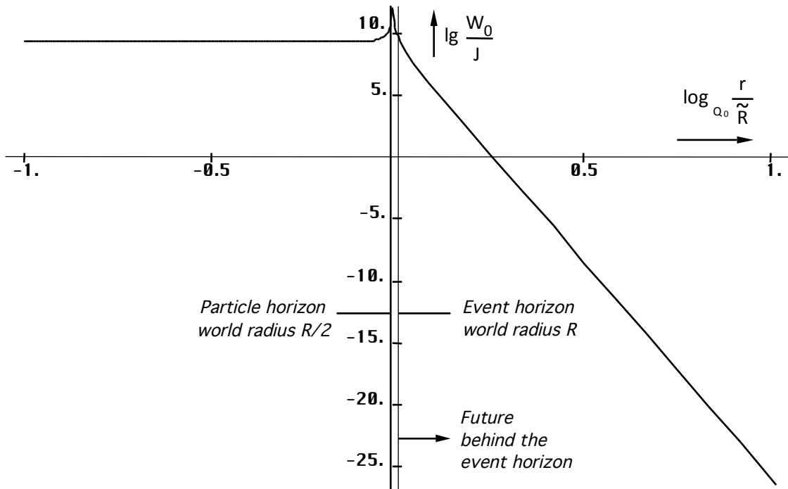
Figure 61 Energy of the Metric line-element spatial dependence up to the event-horizon
