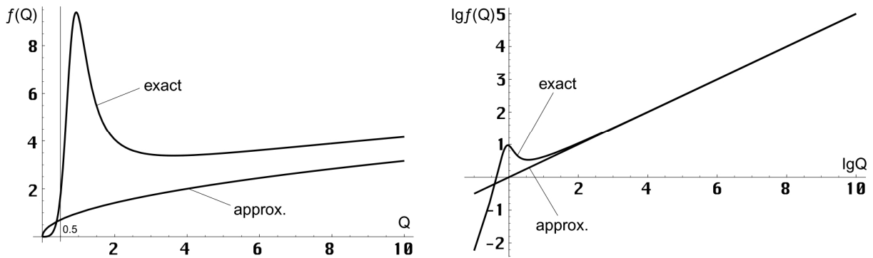
Figure 70 Function BRQ1 exactly and approximation
