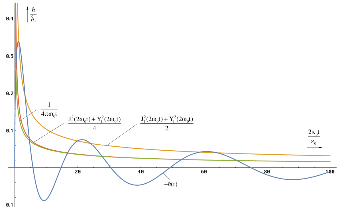
Figure 50 Miscellaneous approximative solutions for PLANCK's quantity of action, larger scale
