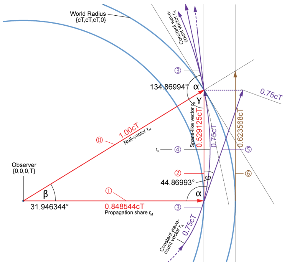
Figure 44b Expansion-velocity and world-radius without correction factor
