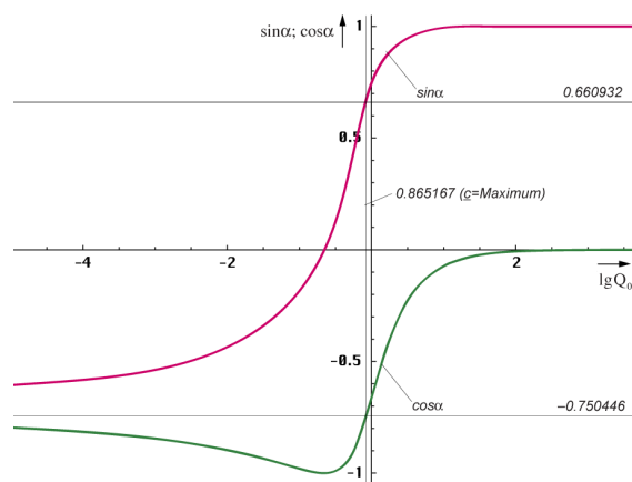
Figure 155 Functions \sin\alpha and \cos\alpha as a function of Q_0
