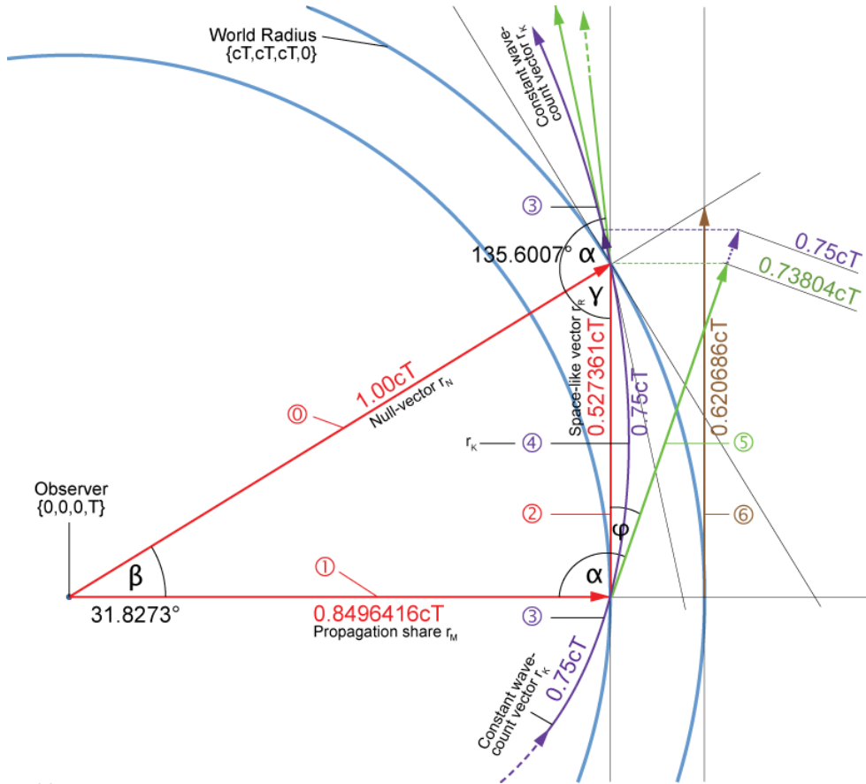
Figure 44a Expansion-velocity and world-radius in the model
