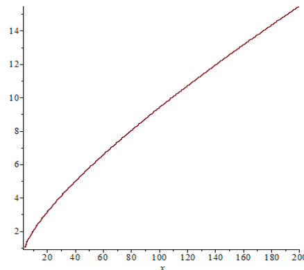
Fig. 1 Discriminant function.
