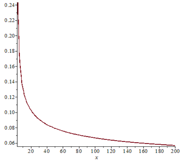
Fig. 2 The first derivative of the discriminant function.
