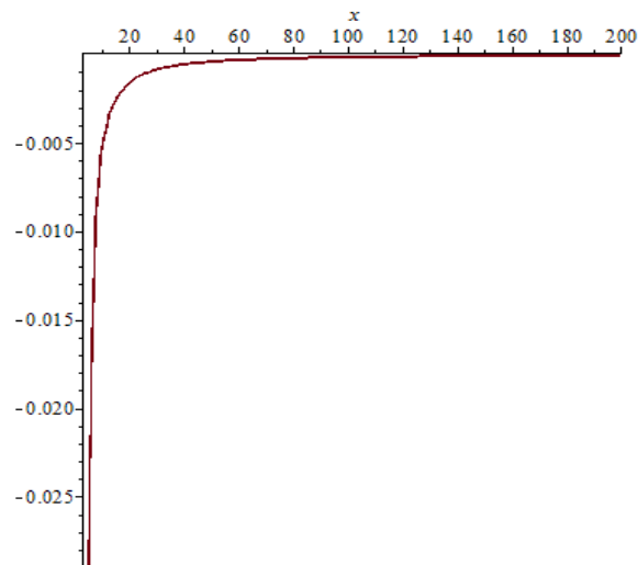
Fig. 3 The second derivative of the discriminant function.
