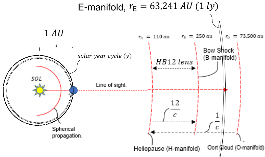
Figure 5: as per based on figure 1, paper 33 ([33]: p9, fig1), calculating the distance of the r_E manifold using the idea of Earth as a solar year ( y ) reference as one revolution around SOL, calculating this value thence as, based on c , 63,241 AU.
