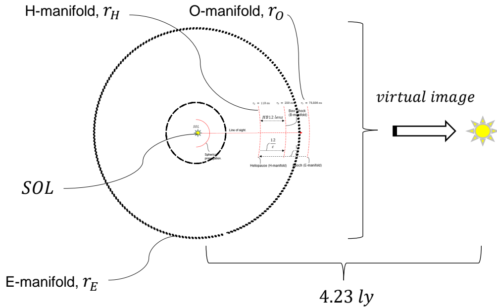
Figure 6: Calculating the light year ( ly ) distance of SOL to the nearest r_E based virtual SOL .
