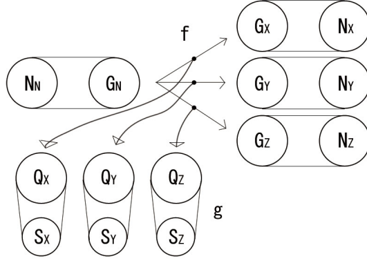
Figure 1: Related Objects
