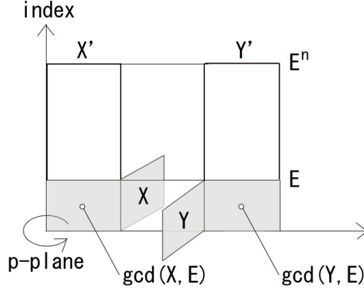
Figure 3: Primes Space
