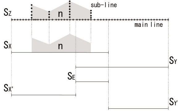
Figure 2: Correspondence Relations
