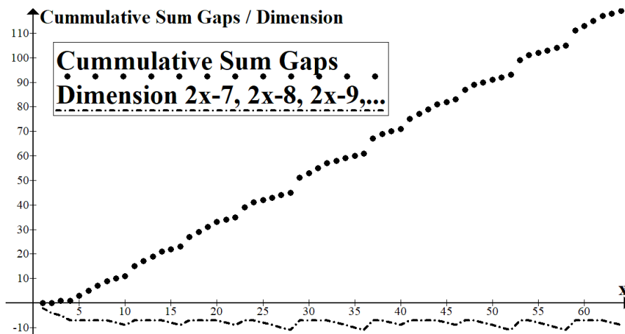
Fig. 25: Prime-Composite finite scale mathematical (graphed) landscape. Data for x = 2 to 64.
