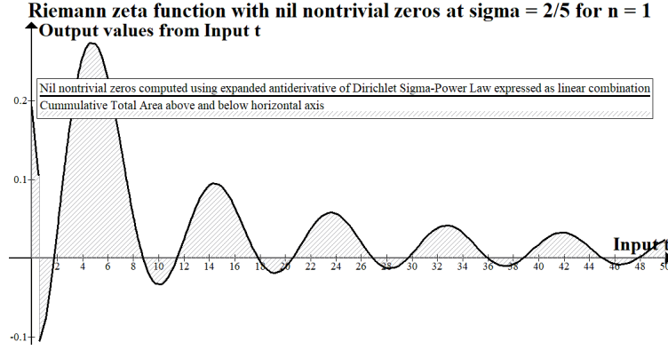
Fig. 13: Nil nontrivial zeros present at \sigma = \frac{2}{5} for n = 1 using Dirichlet Sigma-Power Law.
