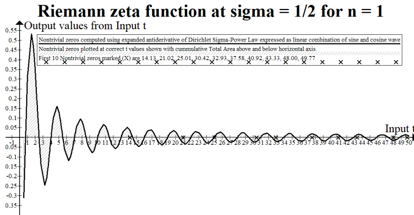
Fig. 10: Nontrivial zeros [first 10 plotted] at \sigma = \frac{1}{2} for n = 1 using Dirichlet Sigma-Power Law.
