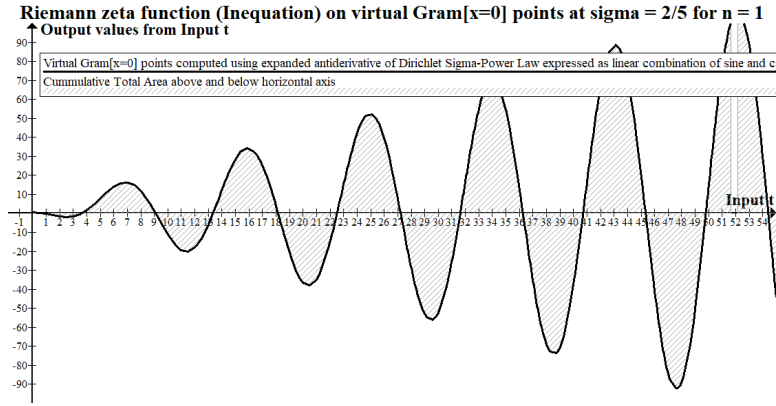
Fig. 22: Gram[x=0] points-Dirichlet Sigma-Power Law as inequation for \sigma = \frac{2}{5} at n = 1 .
