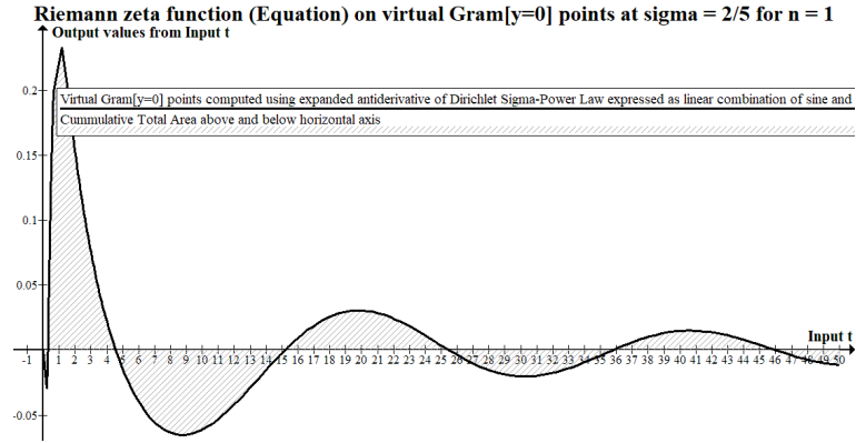
Fig. 19: Gram[y=0] points-Dirichlet Sigma-Power Law as equation for \sigma = \frac{2}{5} at n = 1 .
