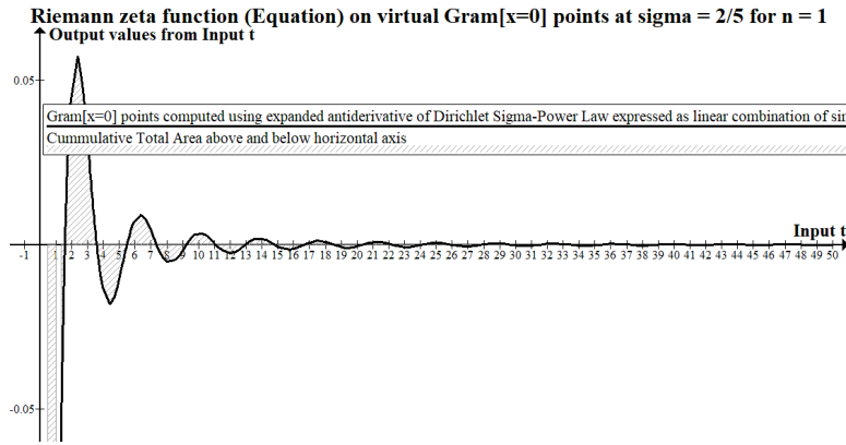
Fig. 21: Gram[x=0] points-Dirichlet Sigma-Power Law as equation for \sigma = \frac{2}{5} at n = 1 .
