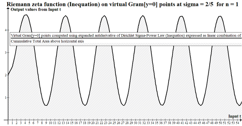
Fig. 20: Gram[y=0] points-Dirichlet Sigma-Power Law as inequation for \sigma = \frac{2}{5} at n = 1 .
