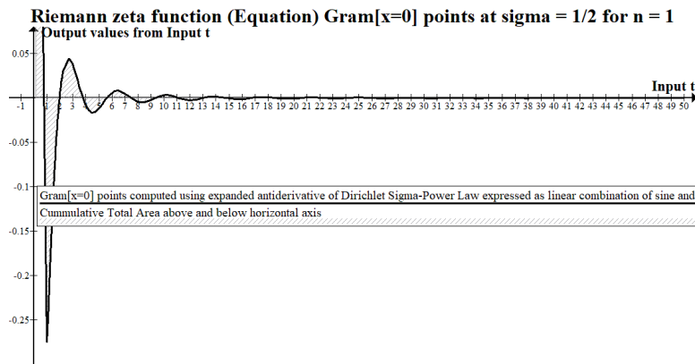
Fig. 17: Gram[x=0] points-Dirichlet Sigma-Power Law as equation for \sigma = \frac{1}{2} at n = 1 .
