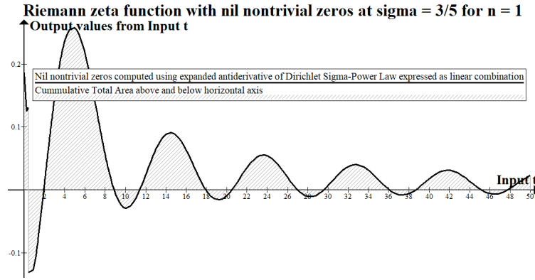
Fig. 14: Nil nontrivial zeros present at \sigma = \frac{3}{5} for n = 1 using Dirichlet Sigma-Power Law.
