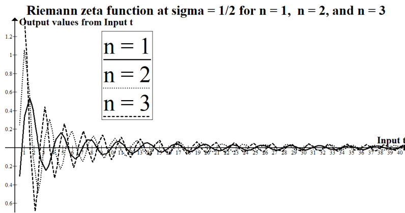
Fig. 11: Nontrivial zeros at \sigma = \frac{1}{2} for n = 1, 2 and 3 using Dirichlet Sigma-Power Law.
