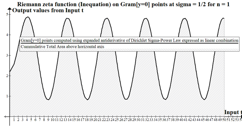
Fig. 16: Gram[y=0] points-Dirichlet Sigma-Power Law as inequation for \sigma = \frac{1}{2} at n = 1 .
