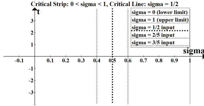
Fig. 6: INPUT for \sigma = \frac{1}{2}, \frac{2}{5}, and \frac{3}{5} . \zeta(s) has countable infinite set (CIS) of Completely Predictable trivial zeros at \sigma = all negative even numbers and [proposed] CIS of Incompletely Predictable nontrivial zeros at \sigma = \frac{1}{2} for various t values.
