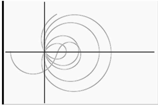
Fig. 7: OUTPUT for \sigma = \frac{1}{2} . Figures 7 represents schematically depicted polar graph of \zeta(\frac{1}{2} + it) plotted along critical line for real values of t running from 0 to 34, horizontal axis: Re\{\zeta(\frac{1}{2} + it)\} , and vertical axis: Im\{\zeta(\frac{1}{2} + it)\} . There are presence of Origin intercepts which are totally absent in Figures 8 and 9 [with identical axes definitions].
