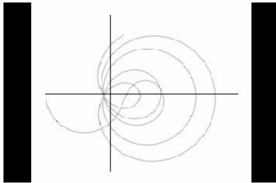
Fig. 8: OUTPUT for \sigma = \frac{2}{3} .
