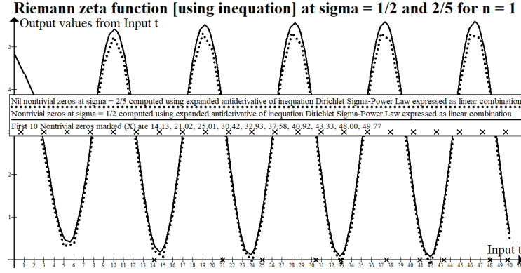
Fig. 12: Nontrivial zeros [first 10 plotted] present at \sigma = \frac{1}{2} and nil nontrivial zeros present at \sigma = \frac{2}{5} for n = 1 using Dirichlet Sigma-Power Law as inequation.
