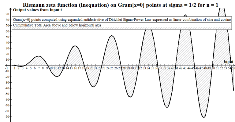
Fig. 18: Gram[x=0] points-Dirichlet Sigma-Power Law as inequation for \sigma = \frac{1}{2} at n = 1 .
