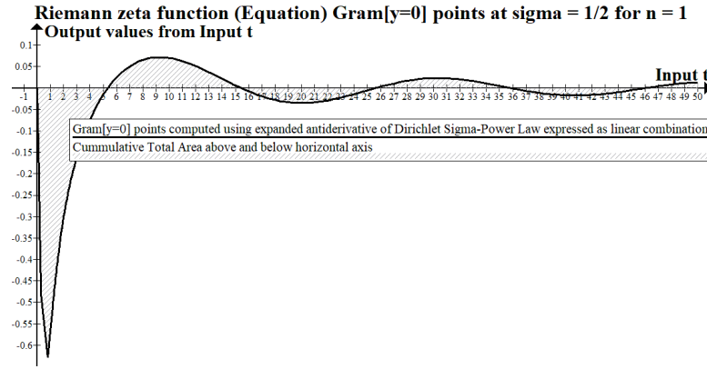
Fig. 15: Gram[y=0] points-Dirichlet Sigma-Power Law as equation for \sigma = \frac{1}{2} at n = 1 .
