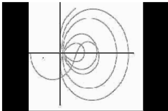
Fig. 9: OUTPUT for \sigma = \frac{3}{5} .
