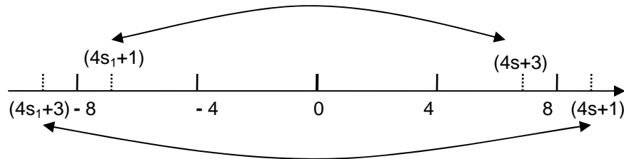
Fig. 2. Symmetrical subsets of odd integer numbers, expressed with a factor of four.
