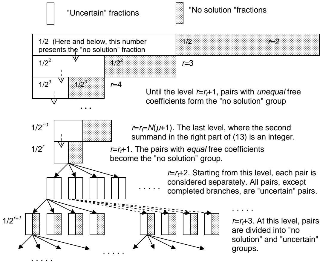
Fig. 1. Graphical presentation of how the "No solution" fraction accumulates through presentation levels, and the appropriate decrease of "Uncertain" fraction. The value of r=r_f=N(\mu+1) is a threshold value, where transition begins from even right parts of equations to integer or rational ones.
