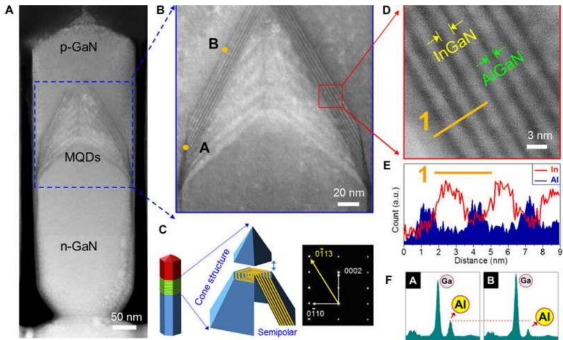
Structural characterization of InGaN/AlGaIn core-shell quantum disk heterostructures. (A) STEM-HAADF image of a representative core-shell InGaN/AlGaIn multiple quantum disk (MQD) heterostructure nanocrystal. (B) High-magnification image taken from the region marked in (A) and (C) schematic illustration for the quasi-3D structure of the semipolar active region and selected-area electron diffraction pattern of the InGaN/AlGaIn core-shell heterostructure. (D) High-magnification HAADF image of the InGaN/AlGaIn quantum disk region. (E) Energy-dispersive x-ray spectroscopy (EDXS) line profile of the InGaN/AlGaIn quantum disks along the line labeled with “1” in (D). (F) EDXS point analysis of the AlGaIn shell region marked as “A” and “B” in (B). Credit: Science Advances, doi: 10.1126/sciadv.aav7523
