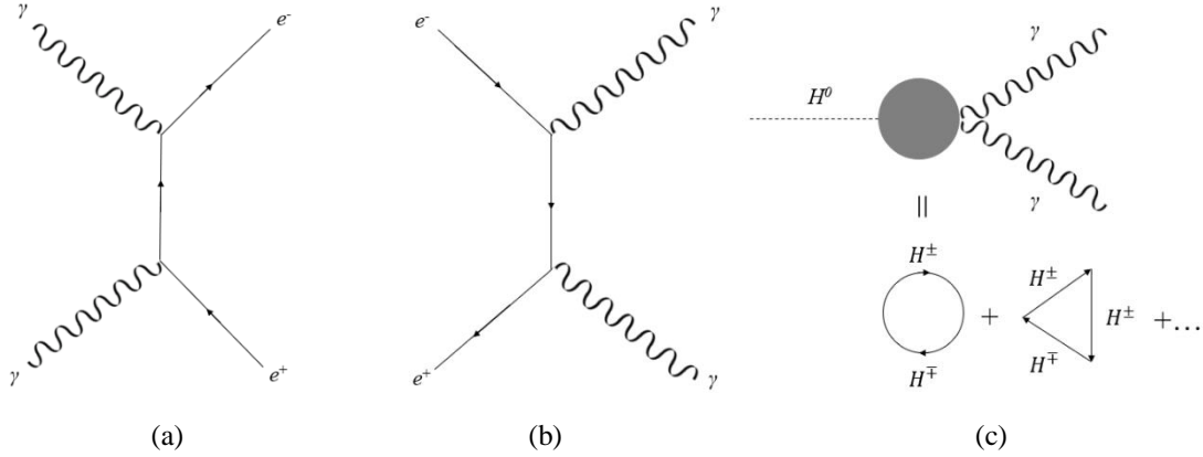
Figure 1. (a) The electron-positron pair production describing in QED. (b) Two-photon production by the electron-positron pair annihilation also describing in QED. (c) The neutral Higgs boson decays to two photons including the parts of vertices [8,9].
