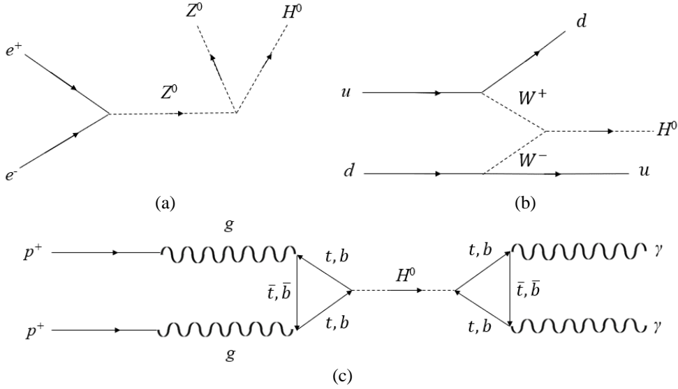
Figure 4. (a) The Feynman diagram for the production of the Higgs boson from the Z gauge boson generated from the annihilation of the electron-positron pair [2]. (b) The Feynman diagram for the production of the Higgs boson from two quarks through the weak interaction [2]. (c) The corresponding Feynman diagram in the biphoton decay from the Higgs boson producing by gluon fusion in two-proton collisions [13] where p is proton, g is gluon, t and \bar{t} are top and anti-top quarks, and b and \bar{b} are bottom and anti-bottom quarks.
