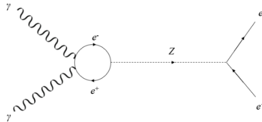
Figure 2. The possible Feynman diagram for two photons through the electron bubble and Z boson intermediates to become to an electron-positron pair.
