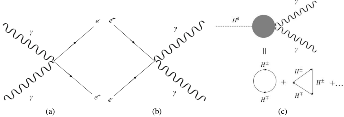
Figure 1. (a) The electron-positron pair production describing in QED. (b) Two-photon production by the electron-positron pair annihilation also describing in QED. (c) The neutral Higgs boson decays to two photons including the parts of vertices [8,9]. The forbidden interaction between the photon field and the Higgs field.
