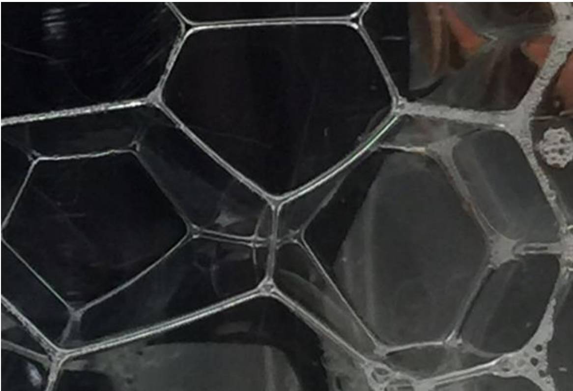
Scutoid cells discovered in soap bubbles
