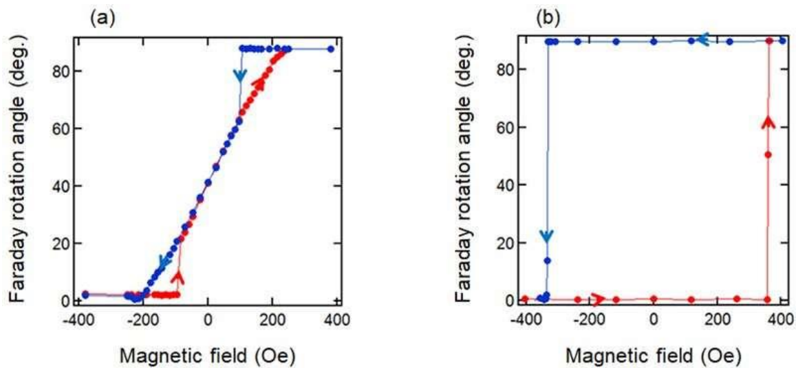
Fig.2 Magnetic field dependence of the Faraday rotation angle measured by the dual-comb magneto-optical effect measurement system. Magnetic hysteresis observed in (a) soft and (b) hard magnetic materials using the dual-comb system. Red and blue points are the measured data when
