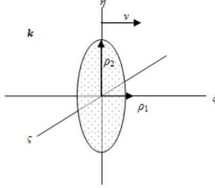
Fig. 4: The radius \rho_2 = c\tau of the expanding light-circle in the \eta - \xi plane (shaded area) is not the same as \rho_1 = c\tau of the light wavefront on the \xi -axis in the direction of motion v , because the respective times \tau are not the same since time depends upon position \xi in system k under Lorentz Transformation from system K .
