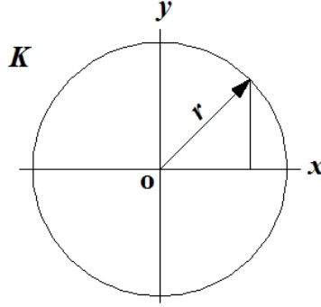
Fig. 2: At any time t the radius r = ct is the same for every position on the x -axis within the light sphere.
