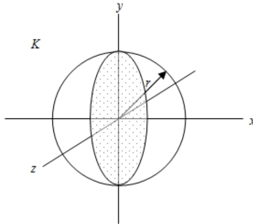
Fig. 1: After a time t > 0 a sphere of light of radius r = ct expands in inertial system K . All positions on the x -axis within the sphere record the same time t and the same radius r = ct . The expanding great circle of light in the y - z plane (shaded area) has the same radius as the wavefront on the x -axis.
