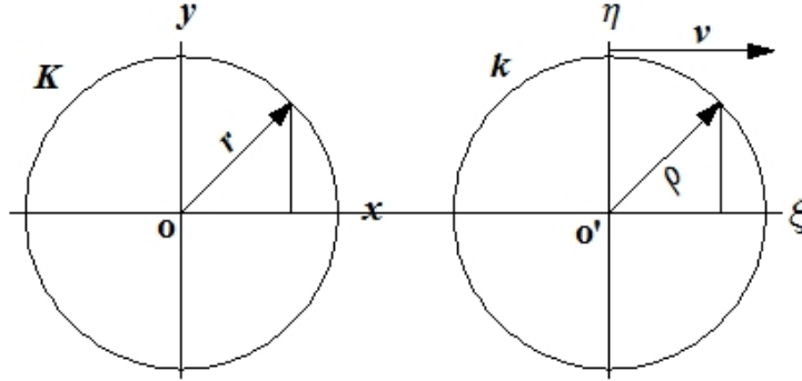
Fig. 3: Einstein's scenario: after a time t > 0 the expanding spherical wave of light has radius r = ct in system K and \rho = c\tau in system k . At t = \tau = 0 the two systems are superposed (so their origins coincide) when the light wave is emitted in all directions. The origins are separated by the distance d = vt according to system K .
