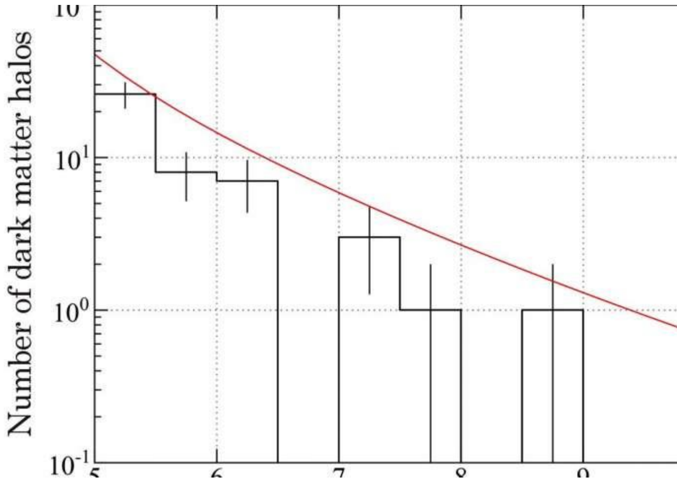
Figure 5: Number of dark matter halos versus their lensing signal strength (black histogram) and number count expected from LCDM and the most recent CMB observation by the Planck satellite. Credit: NAOJ/University of Tokyo [28]
