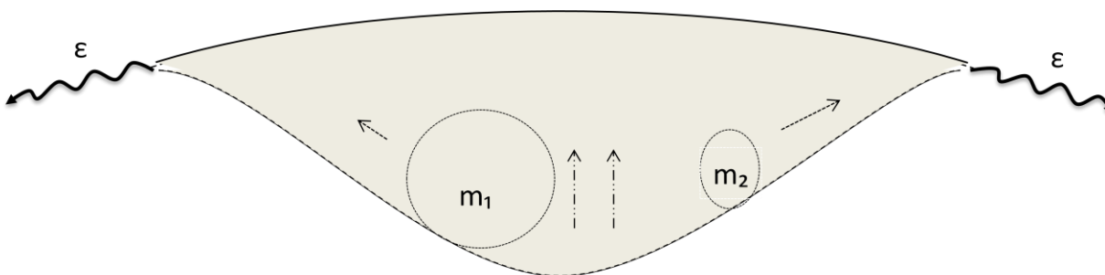
Fig.7: Disintegration of critical mass and the release of another neutrino. (Drawing executed by M.A.)
