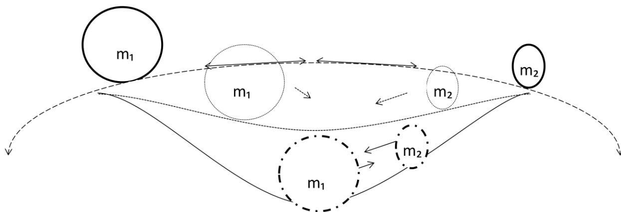
Fig.5: Capitulation of superficial tension of the "space-time membrane", it opposing at dragged of the masses by the process at inflation of the surface. (Drawing executed by M.A.)
