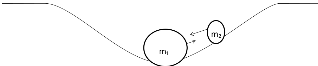
Fig.1: Simplistic interpretation of the gravitational field (which is only attractive) in the presence of the masses. (Drawing executed by M.A.)
