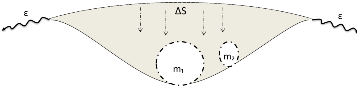
Fig.6: Mechanical work done by the space-time membrane and transmission of oscillation in the whole surface. (Drawing executed by M.A.)
