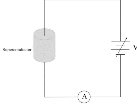
Fig. 4 Another simple electric circuit setup for measuring the electric current A and the resistance or resistivity of the superconductor. The electric voltage V is directly applied on the superconductor.
