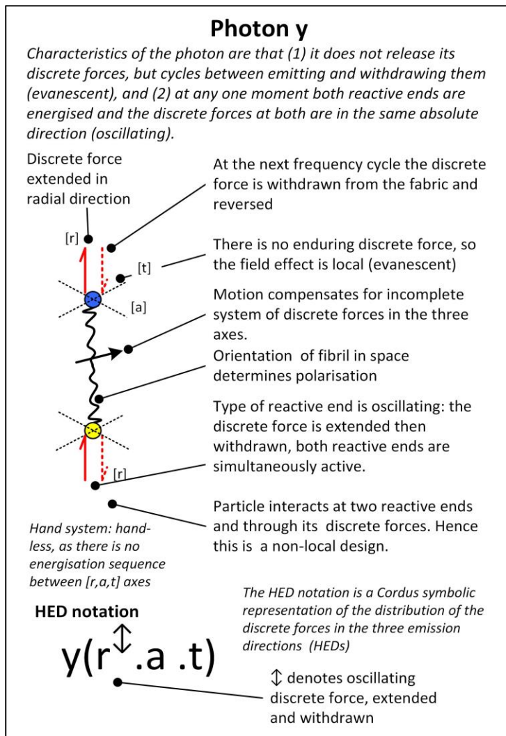
Figure 2: Proposed internal structure of the photon, showing the dual-energisation of the reactive ends, and the shunting arrangement of the discrete forces. Adapted from [28].
