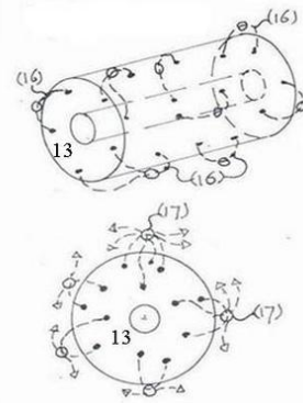
Figure 18, BBBH , the Big Bang Black Hole splintering into smaller BHs and evaporating into the oscillating Axion Higgs Vacuum lattice .
