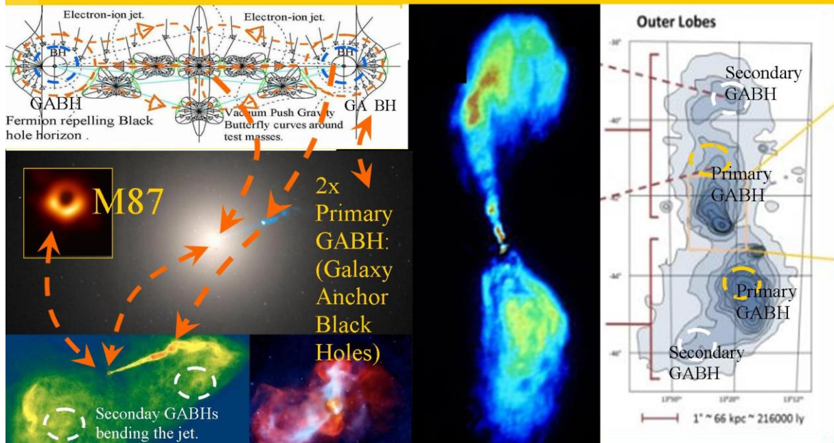
Figure 36, Dual ancient Herbig Haro black holes, called Galaxy Anchor Black Holes, (GABHs) as the origin of M87 and Centaurus galaxies including jets.
