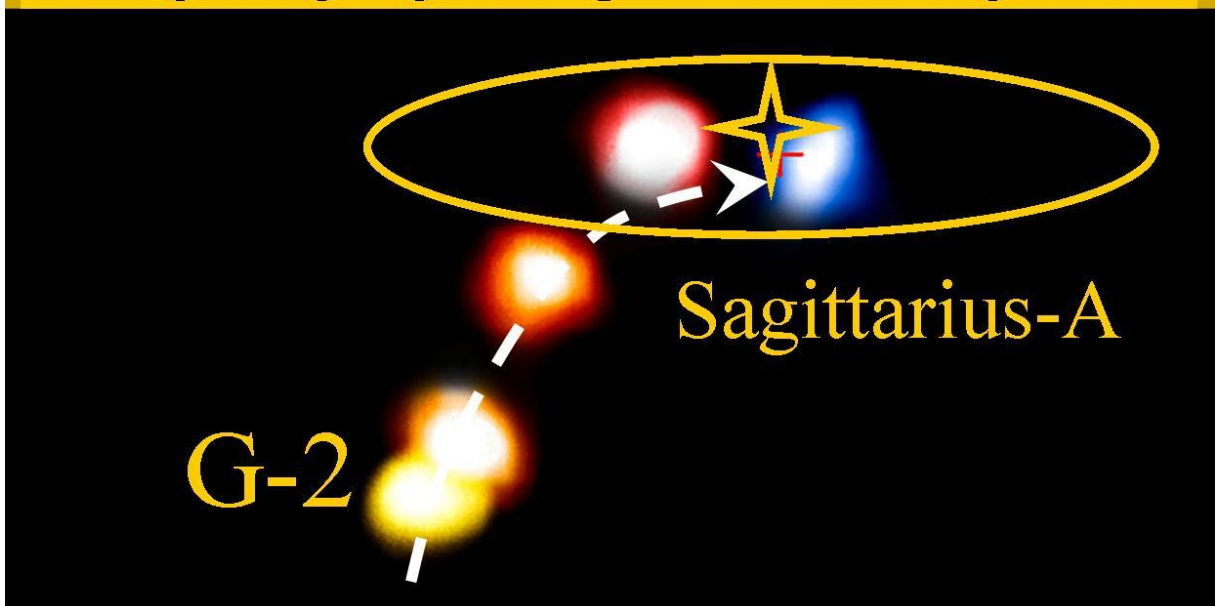
Figure 35, Feeding the Dark Matter Black Hole Dragon ( Sagittarius A) with a smaller black hole ( G2)
