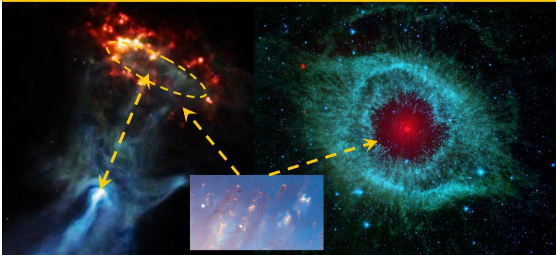
Figure 14, The A-symmetric B 1509-58 nebula , and symmetric Helix nebula as examples of the difference between Fermion and Black hole Quantum Gravity effects.
