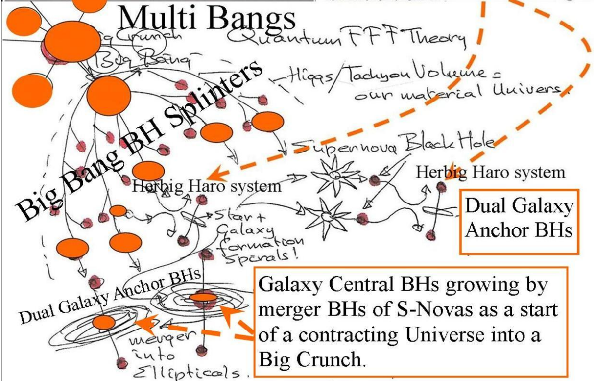
Figure 3, The Multi verse Dark Matter Big Bang Black Hole Splintering into different sized chunks splitting into two equal halves by smaller siblings into equal sized Herbig Haro BH systems.
