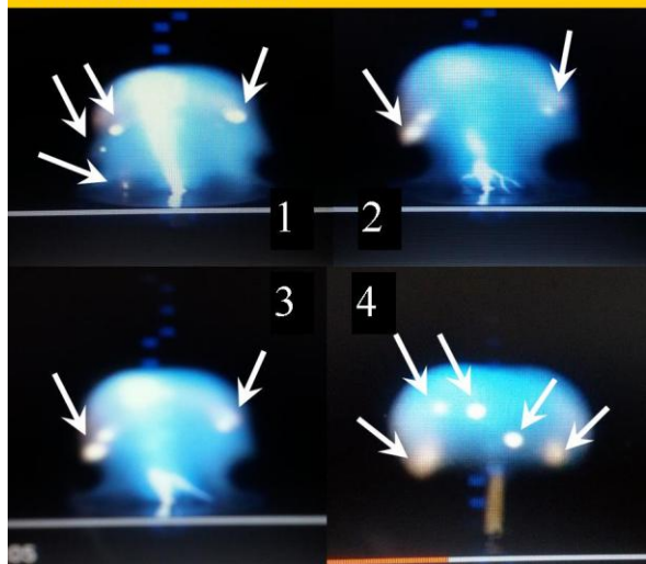
Figure 10 , Microscopic Black Holes on Earth.
