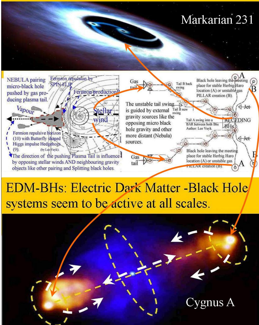
Figure 16. the relation between Markarian 231 and other BH splitting systems
