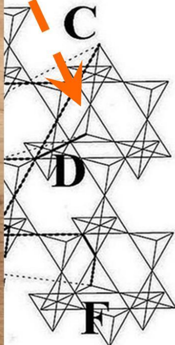
Figure 13 , A stable black hole nucleus is large enough to “eat” the vacuum particles and grow by it.
