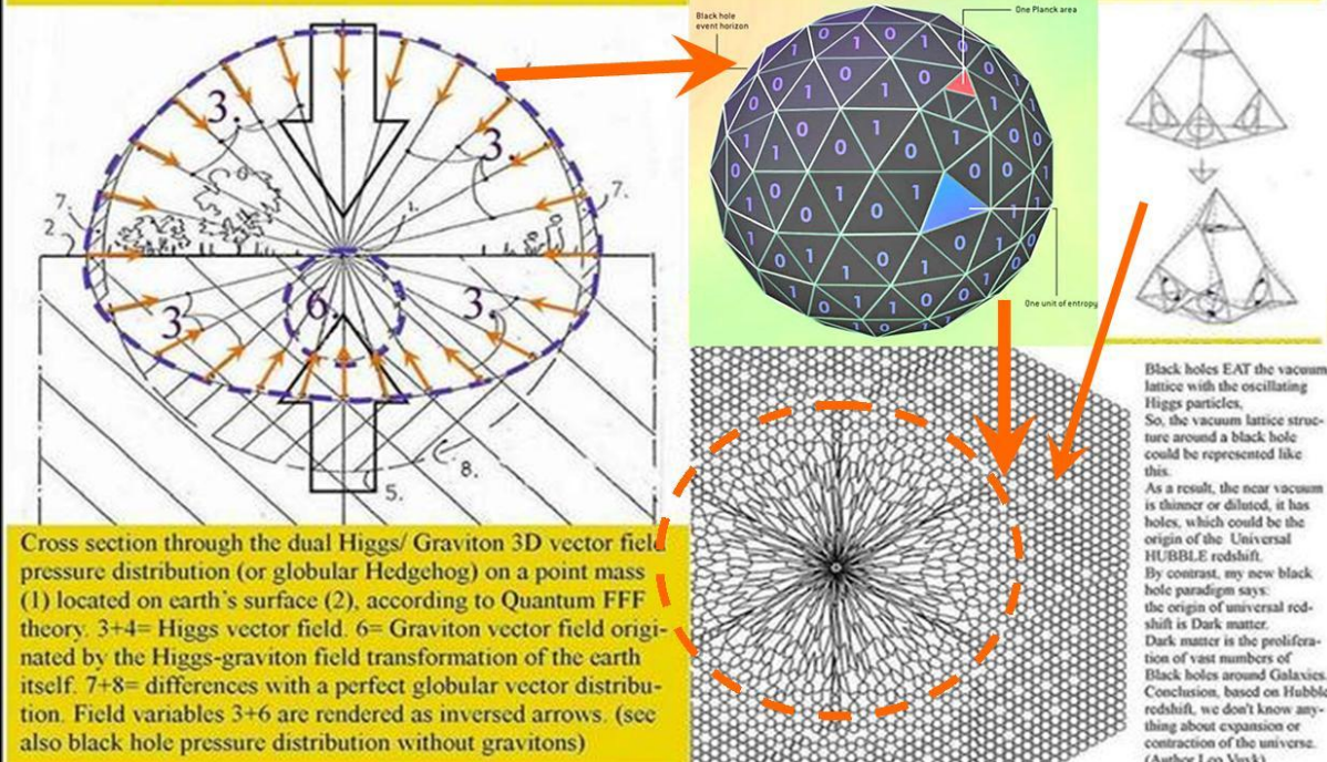
Figure 8. Di-monopole repeller gravity and or entropic emergent gravity combined. Yehuda Hoffmann and Erik Verlinde.
