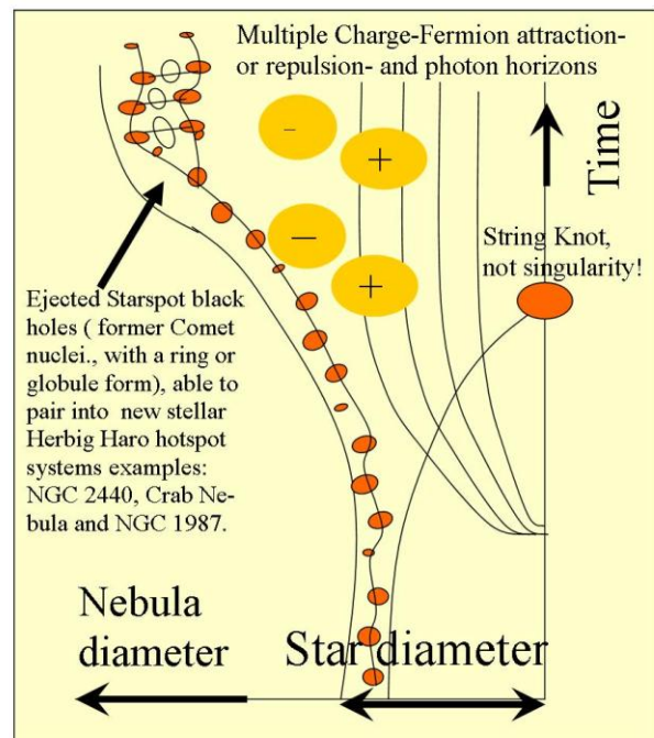
Figure 15 , Other examples of Quantum Gravity effects on ejected rings of micro black hole starspots at work in different nebula .
