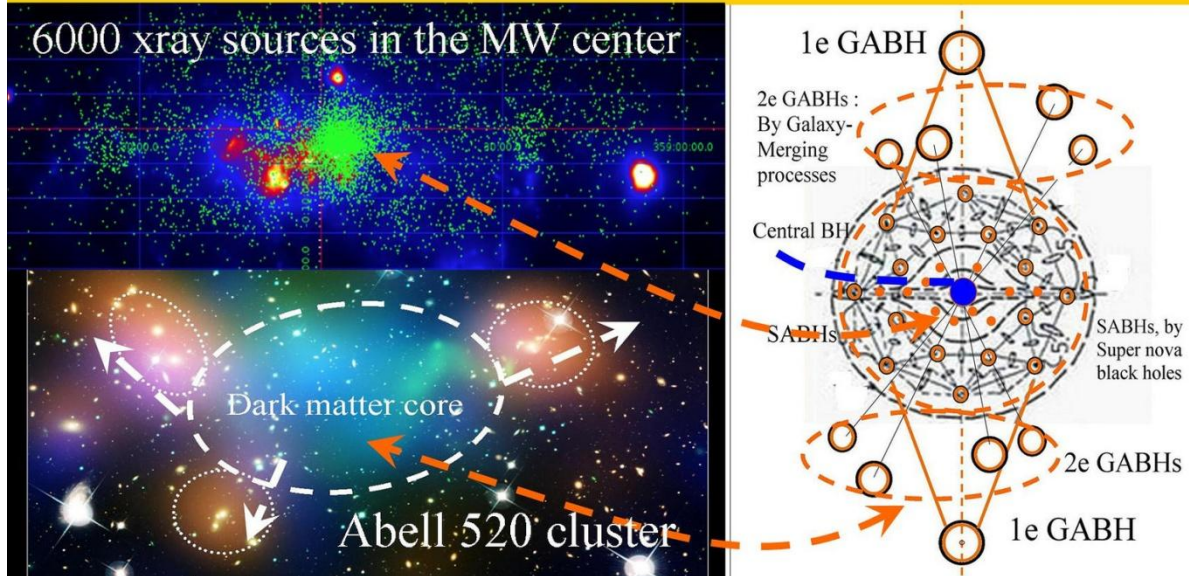
Figure 9, Merger dynamics of NON inertial Dark Matter black holes left behind after merging in the middle.
