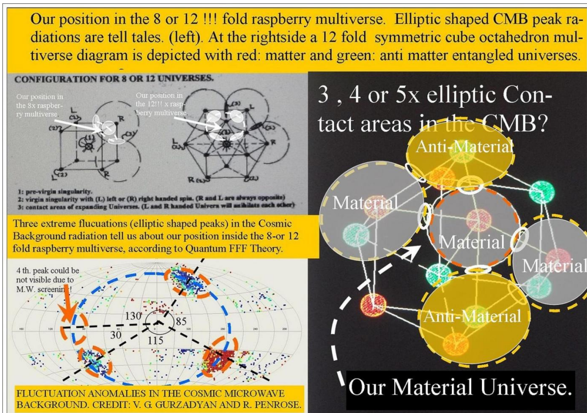
Figure 19, The Multiverse with 8-12 Charge Parity (time) symmetric Universal bubbles.
