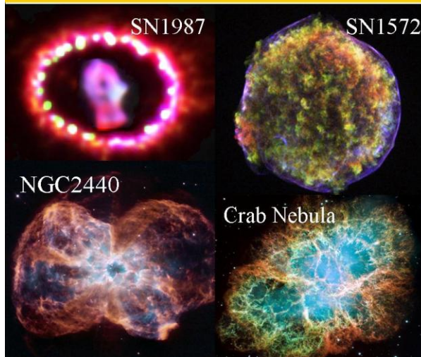
Figure 15 , Other examples of Quantum Gravity effects on ejected rings of micro black hole starspots at work in different nebula .
