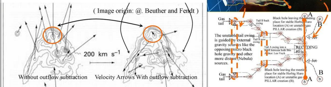
Figure 2. The crucial picture of universal structure creation in a nutshell. Example of NGC 326: The Repelling of Two Equal sized Black Holes as the formation of a HERBIG HARO Bowshock system, with star formation in between and double jets. Below: evidence for New Physics Black Hole inside the Bowshock of a Herbig Haro system, and the splitting of BHs of “pillars of creation”.
