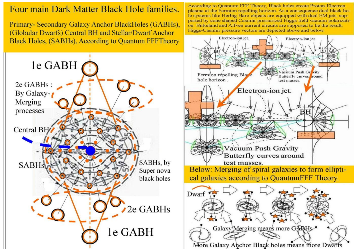
Figure 17, GABHs as the largest unit of Dark Matter black hole families
