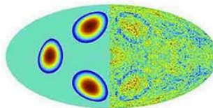
Figure 6 , wavefunction collapse between CP symmetric mirror particles by instant entanglement between multi universal bubbles located around the Big Bang central void.
