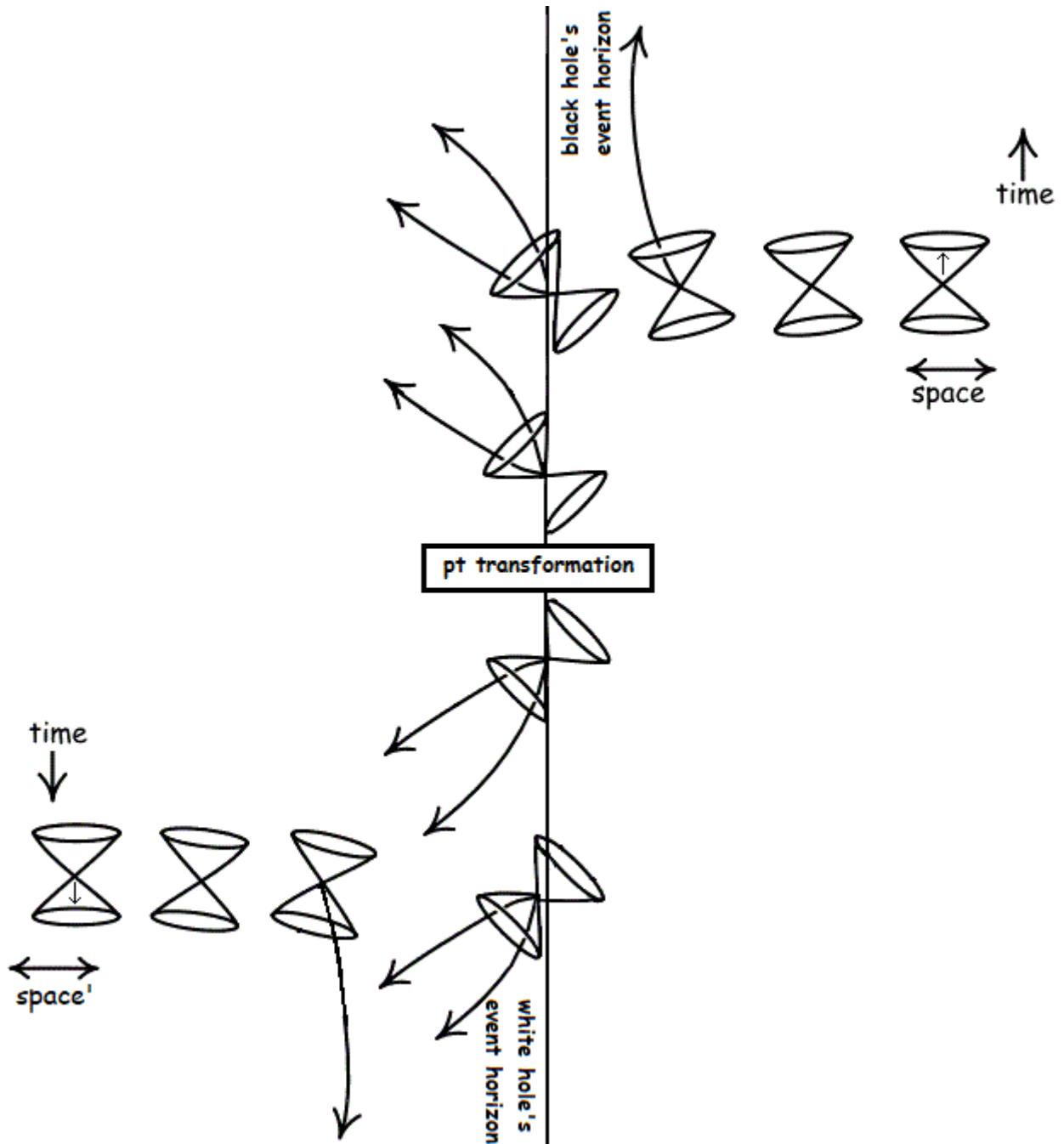
Fig. 2. Light cones evolution (notice that the present time line is divided into different present times for a better description when crossing the horizon, and light cones shape do not change)
