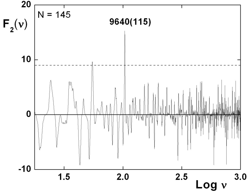
Figure 5. Same as Fig. 4, for the F_2(v) spectrum, computed for N = 145 exoplanets with P < 1.5 days. The strongest peak of the composite commensurability corresponds to a period of 9640(115) s at nearly 3.9\sigma significance (after Kotov, 2018).
