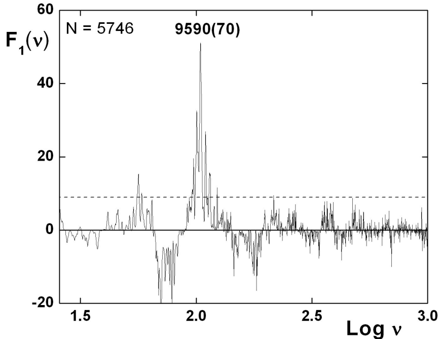
Figure 4. Resonance-spectrum F_1(v) , computed for N = 5746 binaries with periods < 5 days. Horizontal axis gives logarithm of the trial frequency v (in \mu\text{Hz} ), the dashed line indicates a 3\sigma C.L., and the major peak corresponds to a timescale of 9590(70) s.
