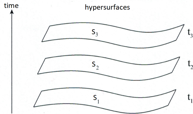
Figure 14.1.: hypersurfaces S_i
