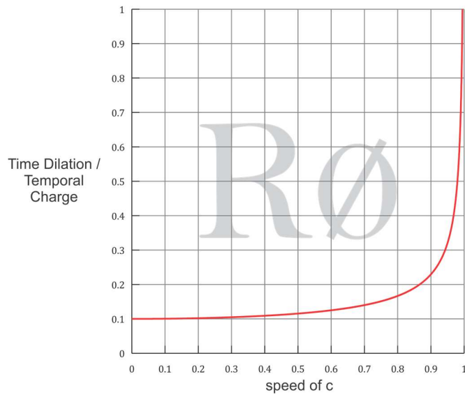
Figure 2. R0 (r-naught)
