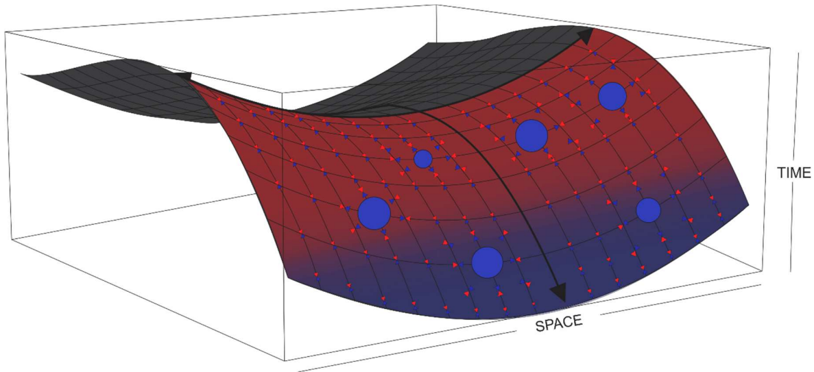
Figure 1. Monopoles of extreme future charge (black holes) attracting past clocks.
