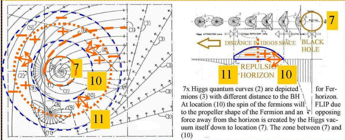
Figure 4, the new Electric Dark Matter Black Hole paradigm.
