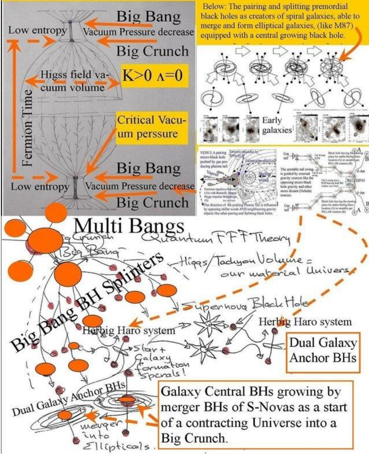
Figure 20, The new Cyclic Multiverse with CP(T) symmetric universes.
