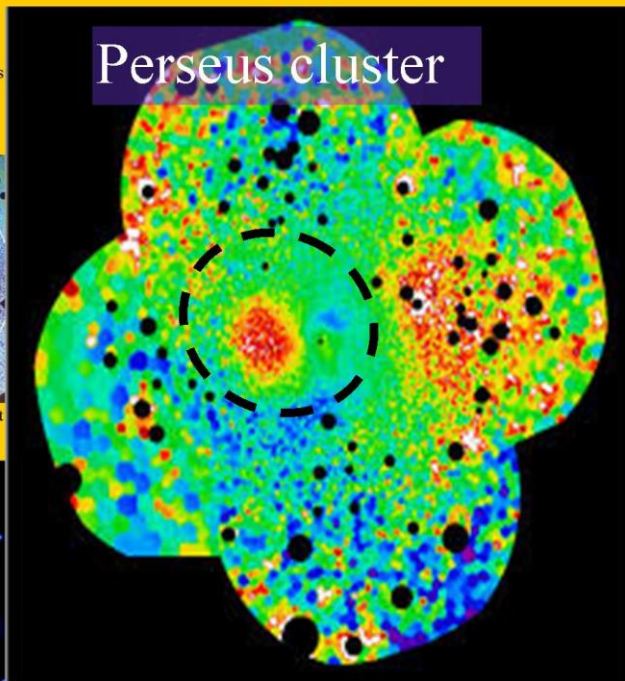
Figure 25, The Smallest black hole are driven into the center of galaxies.
