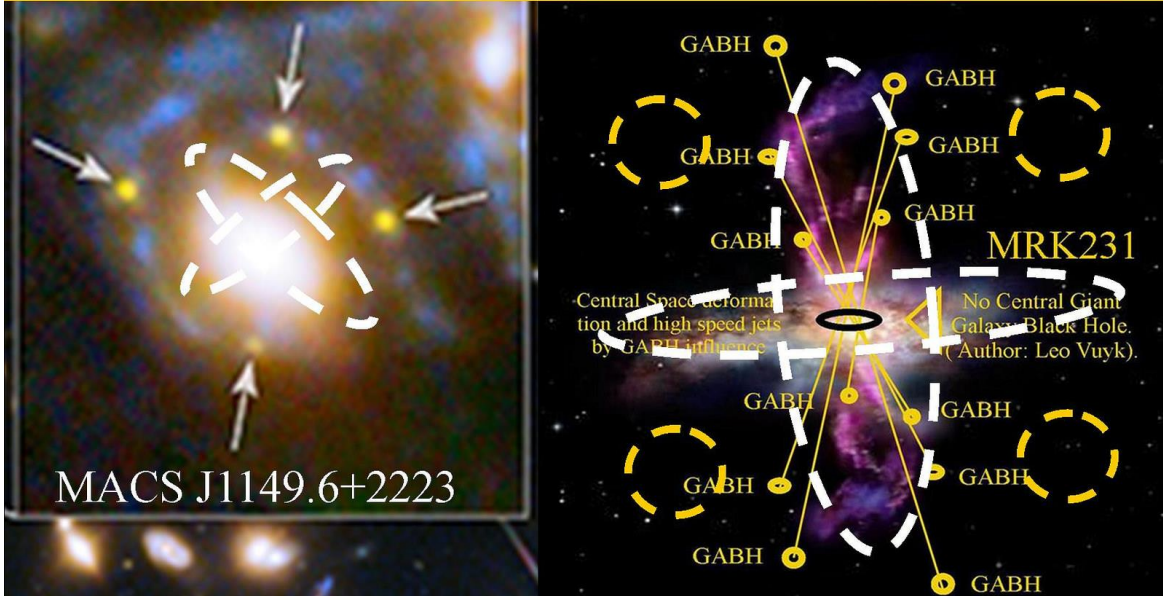
Figure 27. Quadrupole dark matter distribution based on one or even two spiral galaxies observed “edge on”.
