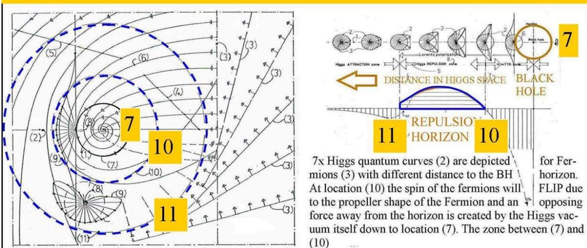
Figure 16, The principle of fermion production (also water) and repulsion around a new paradigm black hole.
