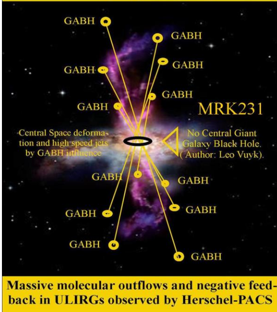
Figure 21, Primordial Galaxy Anchor black holes.
