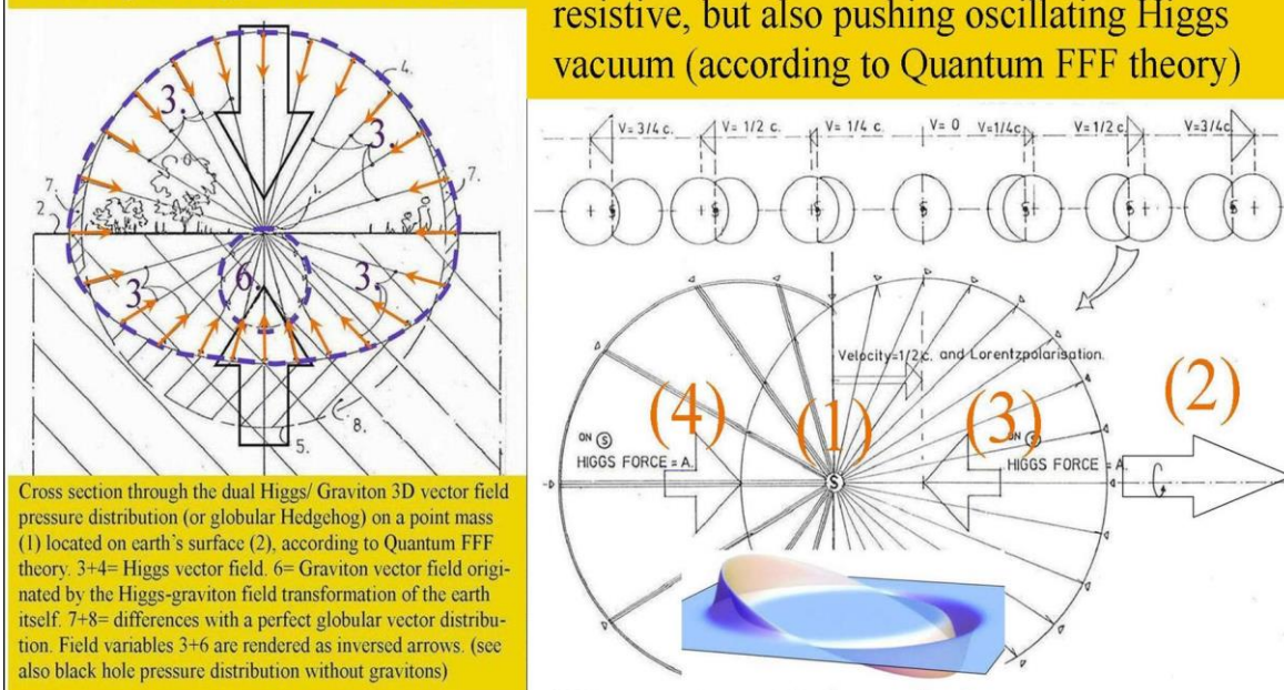
Figure 19, equivalence between gravity and acceleration does not hold in Q-FFF theory.
