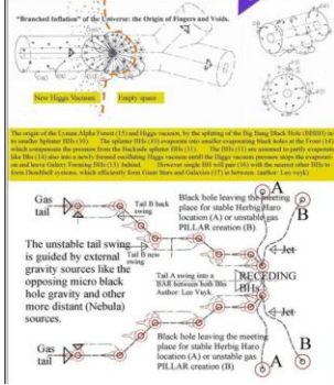
Figure 22, star formation and dying according to Quantum-FFF Theory.
