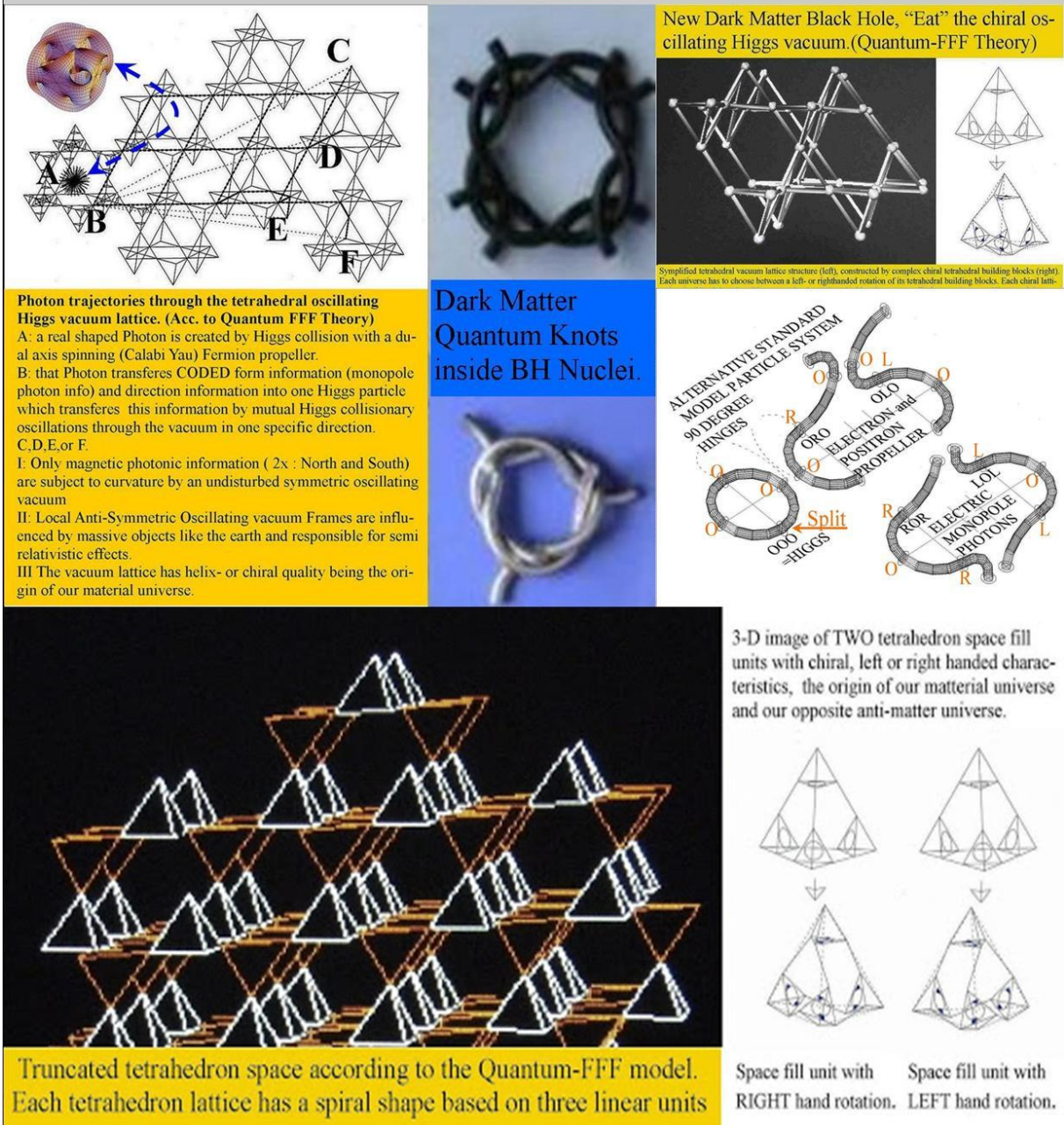
Figure 9, Dark energy vacuum field with topological superconductor function for local and inter-universal entanglement as a base for particle wave function collapse, consciousness and democratic free will according to Quantum FFF Theory.
