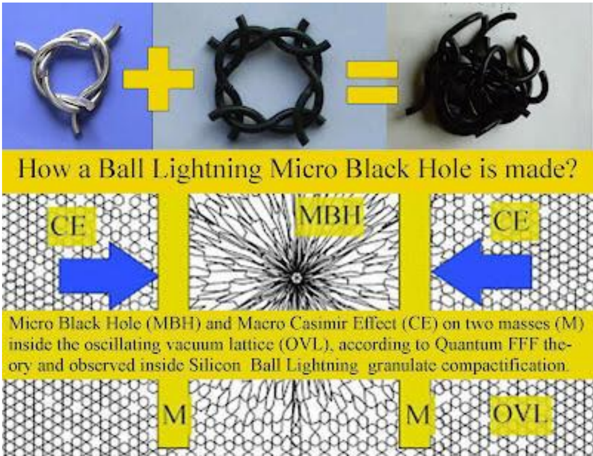
Figure 7, basic Higgs elements for black hole formation, with vacuum deformed structure around a black hole.
