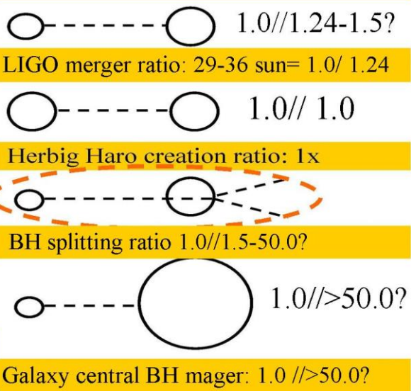
Figure 8, suggestions for black hole nuclear splitting by BH collision.
