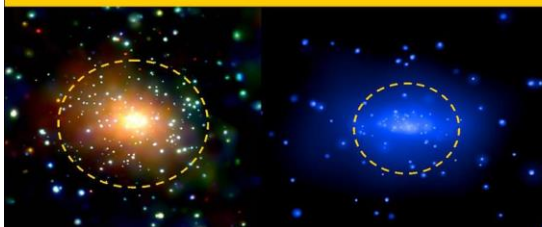
Figure 25, The Smallest black hole are driven into the center of galaxies.
