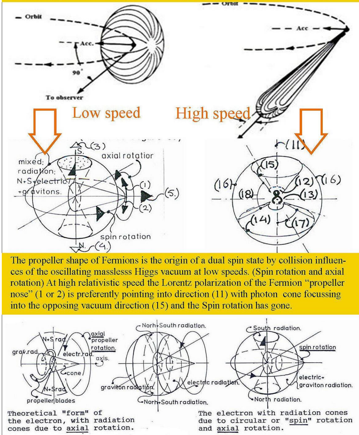
Figure 28, Propeller shaped Fermions and the synchrotron effect.
