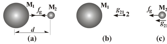
Fig. 0-22. Gravitational field.
