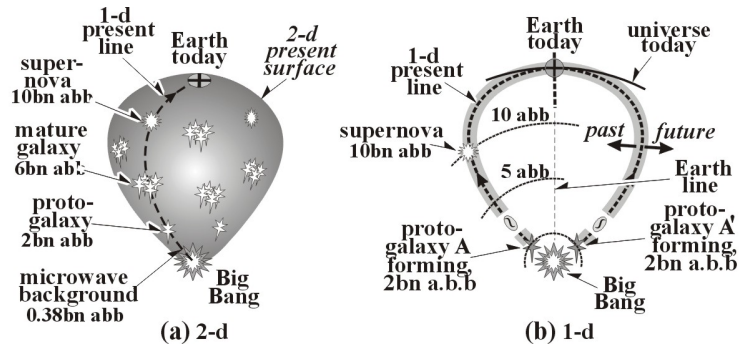
Fig. 0-18. Present surface.
