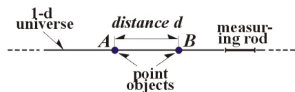
Fig. 0-2. Distance.
