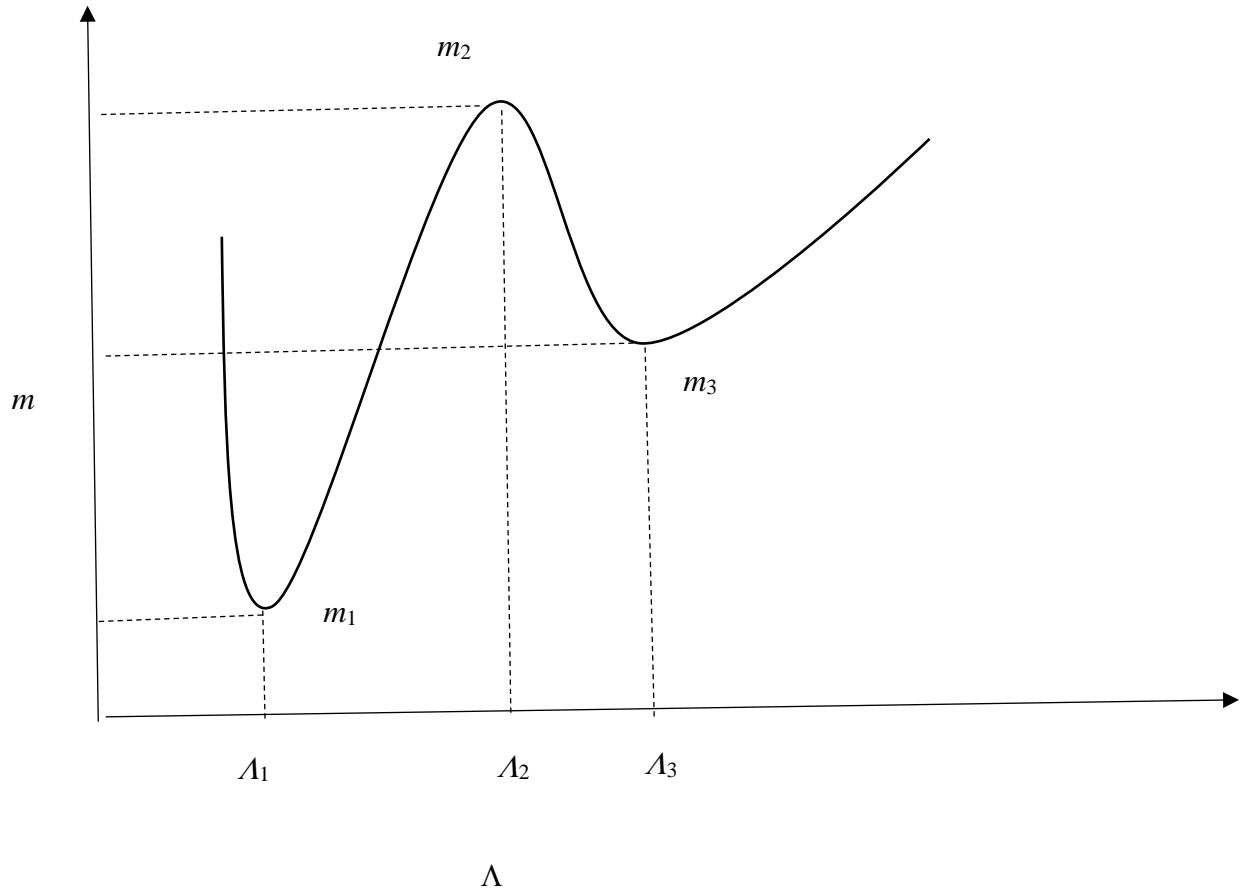
Fig.1. Sketch showing minimum m_1 representing masses of electron, up quark or down quark; a maximum m_2 corresponding to masses of tau lepton, top quark or bottom quark and second minimum representing masses of muon, strange quark or charm quark taken that order ( figure not drawn to represent the scales involved)
