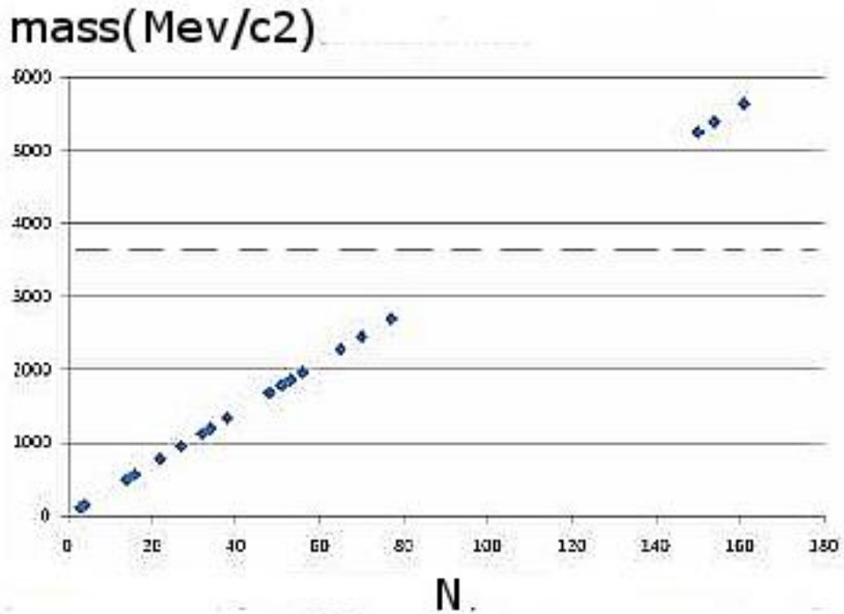
Figure 3: This plot shows all baryons and mesons with lifetimes greater than 10^{-24} sec. [12]( see text for details). The traced line indicates the calculated 3710 \text{ Mev}/c^2 , which is in the expected range of energy for a parent-state for the particles below it.
