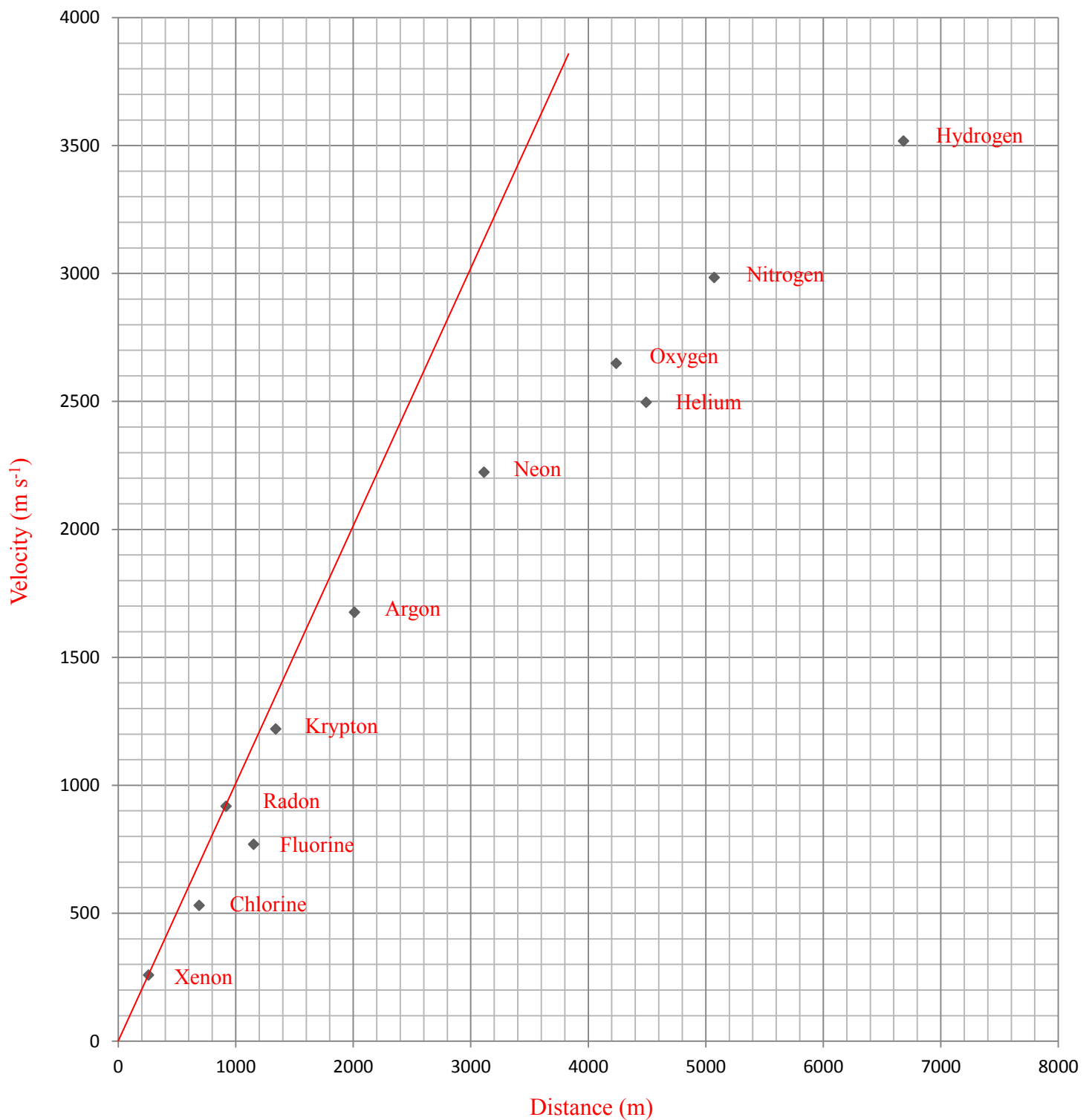
Figure 8. Velocity-distance relation plot for gas molecules expanding differentially (differential molecular expansion) (Table 8). Local molecules, Xenon and Radon are allowed to expand at the same time and therefore they exhibit a linear-velocity distance relation. The remote molecules are allowed to expand differentially and therefore they deviate from exhibiting a linear velocity-distance relation. Such differential expansion causes the distance of remote molecules to be larger than expected with respect to the local molecules without any acceleration. In other words, expansion initiated for the remote molecules before it did for the local molecules.
