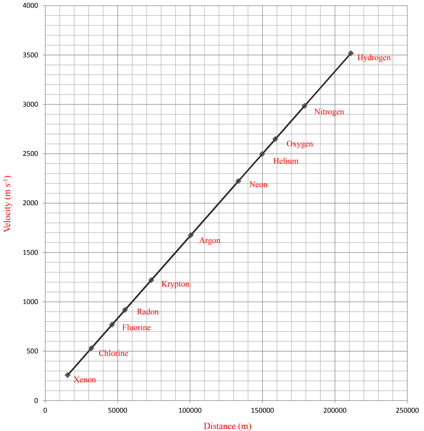
Figure 6. Velocity-distance relation plot for molecules expanding at very high temperature with large differences in temperature. Observation time = 60 seconds ( Table 6 )
