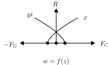
Fig. 8: Complex plane for the image set
