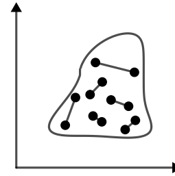
Fig. 3: Conservative area with a random closed curve
