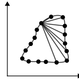
Fig. 4: Creating mass
