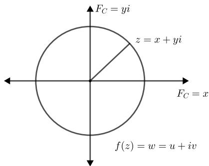
Fig. 7: Complex plane
