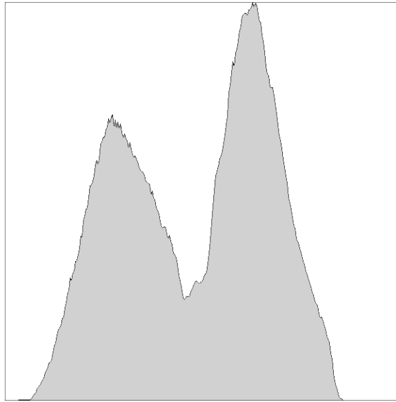
Figure 7: Displacements of Z' = \sin(Z) + C \sin(Z) , where C_{xyzw} = 0.3, 0.5, 0.4, 0.2 . For this histogram the maximum displacement is 3.93216; mean: 2.22363; mode: 2.45514; standard deviation: 0.866331; variance: 0.75053; skewness: -0.175938 ; kurtosis: -1.22836 .
