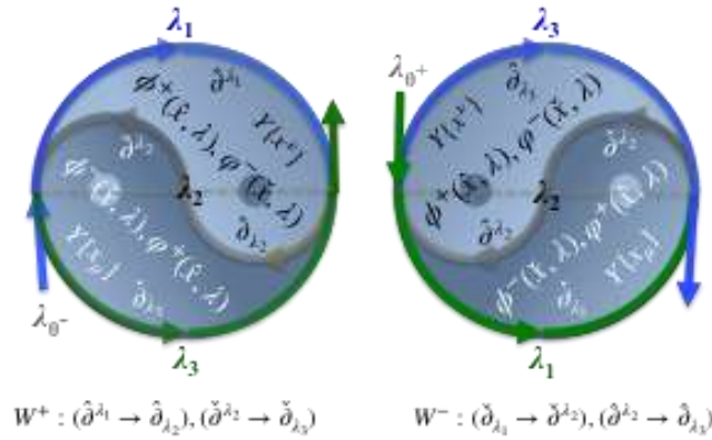
Figure 4a: Event Flows of Y^-Y^+ Evolutional Processes \hat{\partial}^\lambda \cup \hat{\partial}_\lambda \equiv \check{\partial}^\lambda \cup \check{\partial}_\lambda
