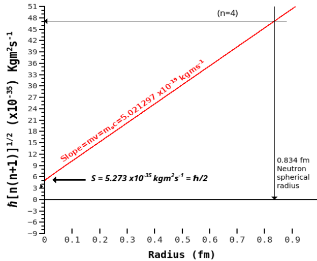
Figure 6: Prediction of the neutron radius.
