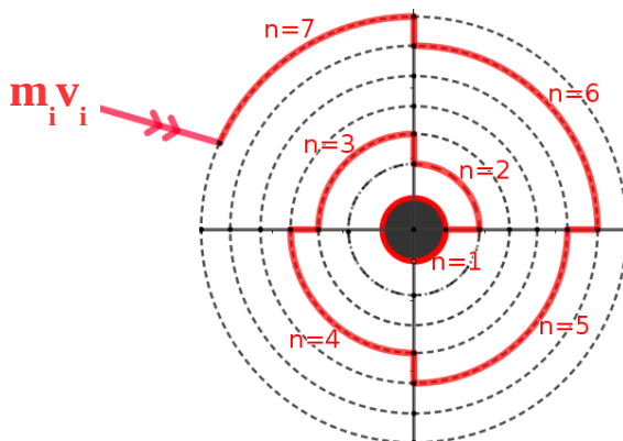
Figure 1: Initial momentum m_i v_i entering spiral motion for particle creation. Discrete orbitals are shown in red for angular quantum numbers n=7 to n=1 .
