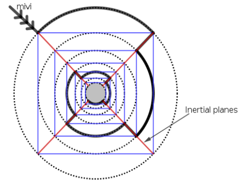
Figure 6: Proposed Inertial Planes
