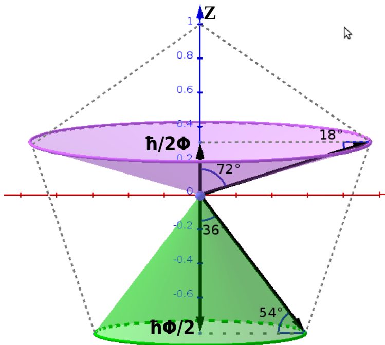
Figure 5: The proton spin angular momentum \pm\hbar/2 as the resultant of two opposing momentum \hbar/2\Phi and \hbar\Phi/2 , perfectly fitting an equilateral pentagon.
