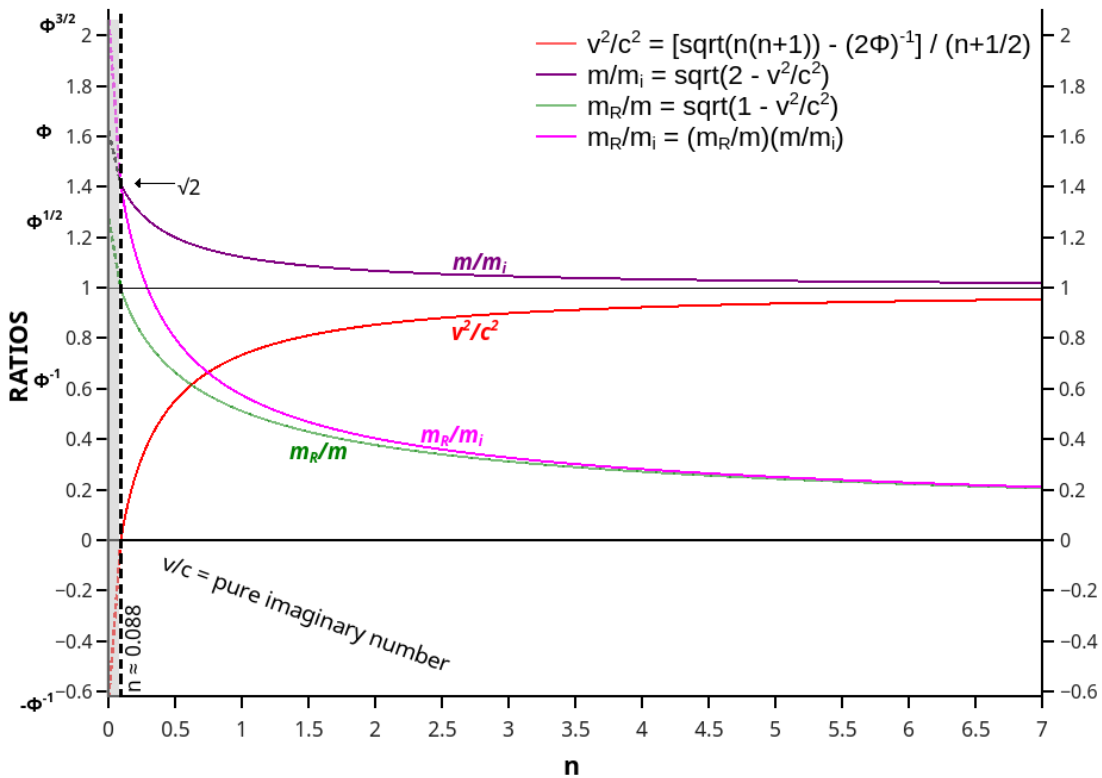
Figure 4: Graph showing the behaviors of the ratios v^2/c^2 , m/m_i , and m_R/m_i during the down-spiral of the initial linear momentum m_i v_i with m_R standing for the mass at tangential velocity=0
