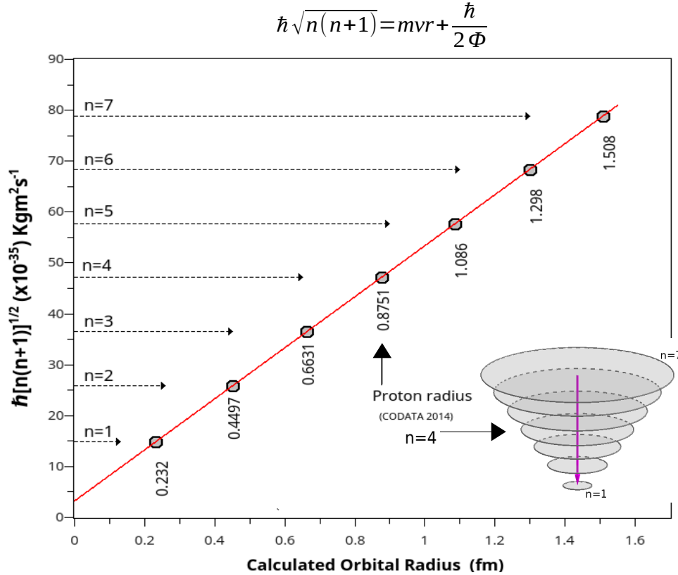
Figure 3: Determination of the orbital radii from n=1 to 7, with n=4 corresponding to the proton radius 0.8751 fm.
