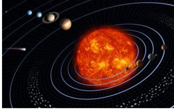
Fig. 1. Solar system, top view.
